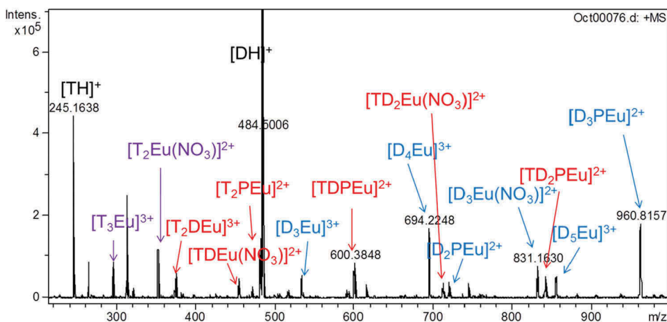
Figure 7. ESI-MS spectrum of DMOHEMA 3.10^{-3} mol.L ^{-1} , HDEHP 1.5.10^{-3} mol.L ^{-1} , TEDGA 1.5.10^{-3} mol.L ^{-1} , Eu 1.5.10^{-3} mol.L ^{-1} and HNO _3 3.10^{-3} mol.L ^{-1} diluted ten times in acetonitrile/water (50-50% vol.), positive ionization mode, (D = DMOHEMA, HP = HDEHP, T = TEDGA).
