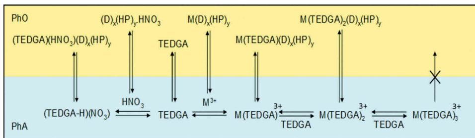
Figure 8. Schematic view of complexation equilibria and extraction mechanisms involving TEDGA in the biphasic system DMDOHEMA (D), HDEHP (HP)/HNO _3 , TEDGA, Ln/Am (M).
