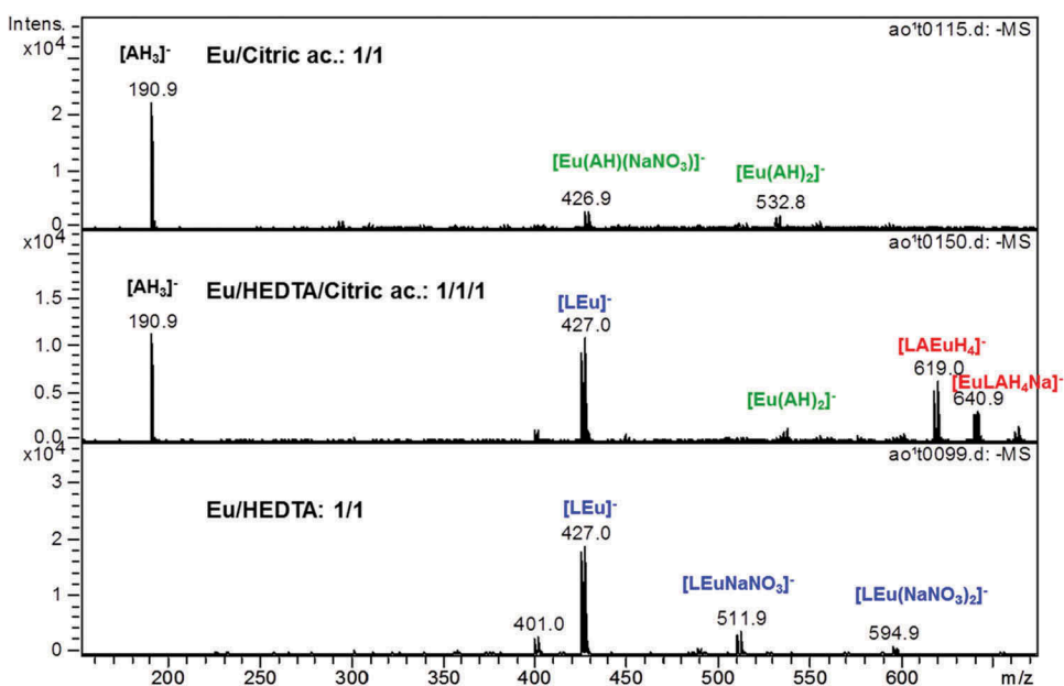
Figure 10. ESI-MS spectrum of Eu/citric acid, Eu/HEDTA, and Eu/HEDTA/citric acid solutions ( \text{A}^- : unprotonated citric acid, \text{L}^- : unprotonated HEDTA), negative ionization mode.
