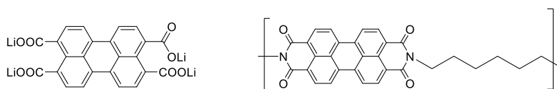
Figure 1: Lithium perylene-3,4,9,10-tetracarboxylate and Polyhexamethylene-peryene-3,4,9,10-tetracarboxylic diimide
