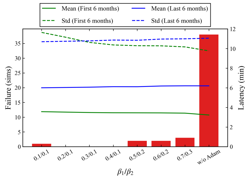
Figure 12. Latency and number of failed simulations of LAC-AB algorithm.
