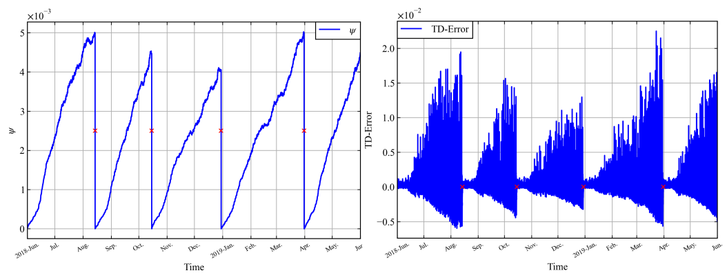
Figure 5. Divergences of \psi (left) and TD-errors (right) over one year with the state-of-the-art LAC method (red crosses indicate the power failure points).
