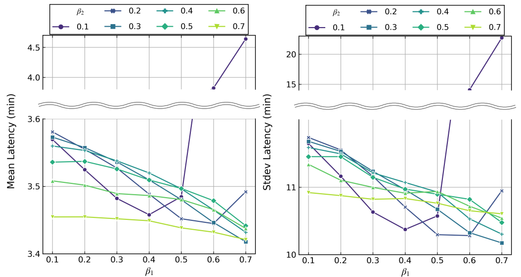
Figure 9. Latency analysis of LAC-AB during the first six months for different sets of (\beta_1, \beta_2) using EHD1 dataset: (left) mean; and (right) standard deviation.
