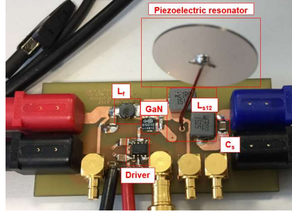
Fig.6 Experimental class L-Piezo inverter
