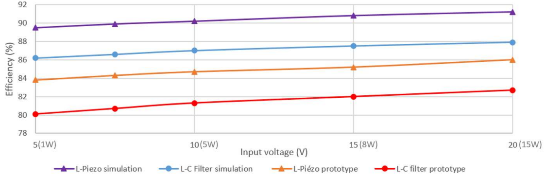
Fig.9 Efficiency comparison between L-Piezo simulation, L-C filter simulation, L-Piezo prototype and L-C filter prototype in the 5V \leq V_{in} \leq 20V range
