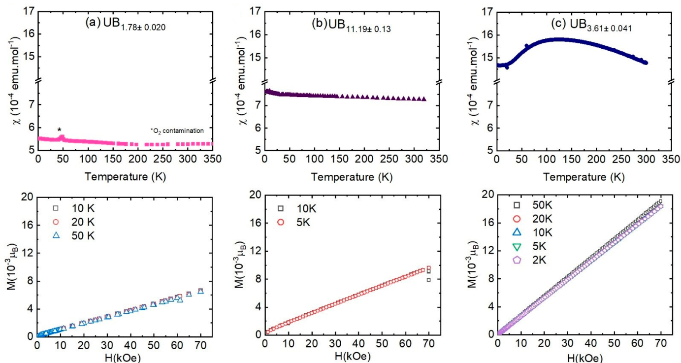
Figure 3. Magnetic susceptibility curves against temperature (top) and magnetization against field (bottom) for (a) \text{UB}_{1.78} , (b) \text{UB}_{11.19} , and (c) \text{UB}_{3.61} .
