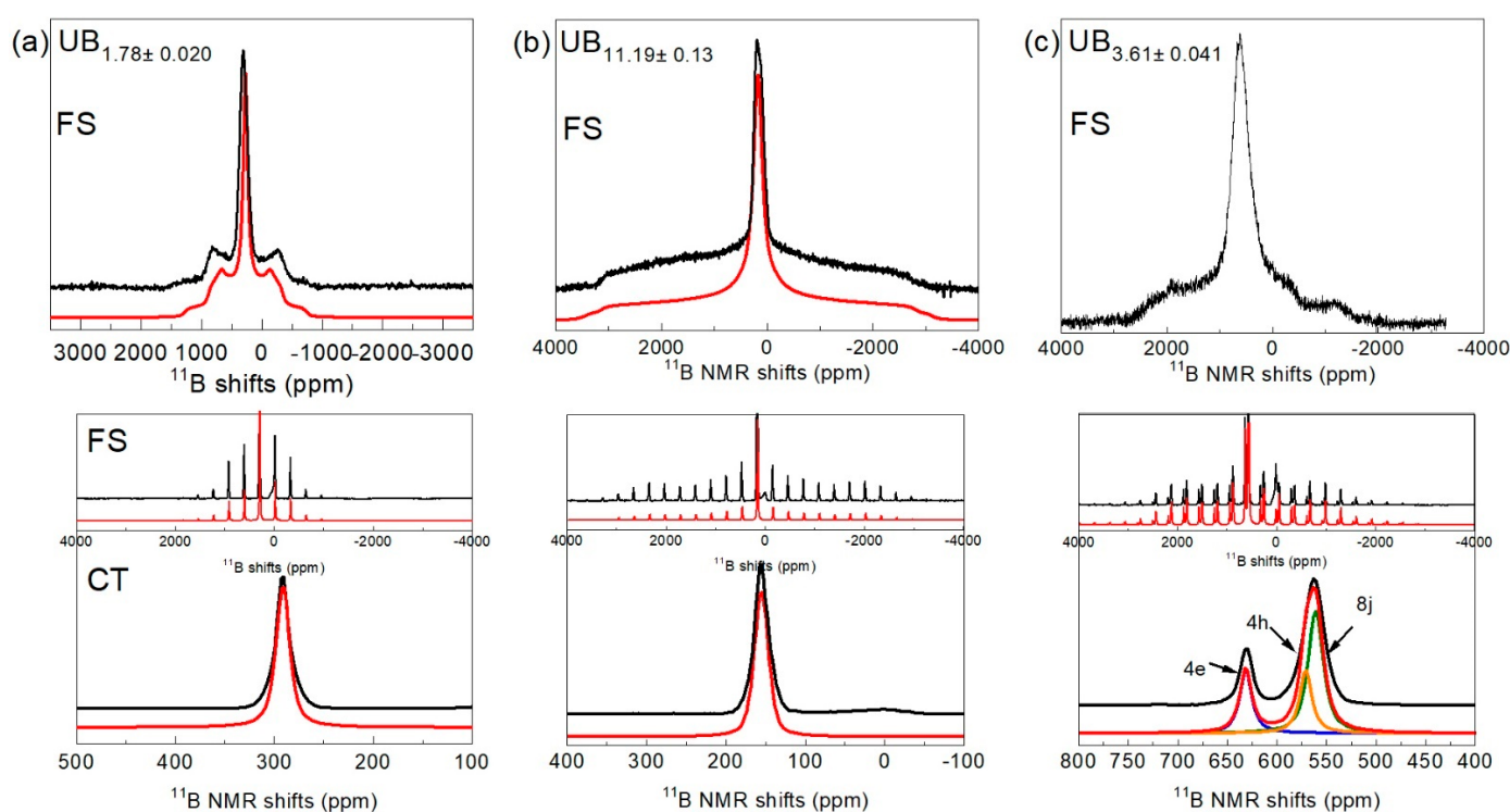
Figure 4. ^{11}\text{B} static (upper) and MAS-NMR spectra (lower) for (a) \text{UB}_{1.78} , (b) \text{UB}_{11.19} , and (c) \text{UB}_{3.61} showing the central transition (CT) and the Full spectra (FS). The fits are the red lines.
