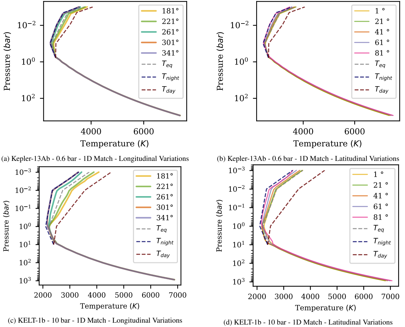
Fig. 4. Snapshots of the latitudinally ( left ) or longitudinally ( right ) averaged T - P profile for two evolved models of Kepler-13Ab ( top ) and KELT-1b ( bottom ), both with a very shallow horizontal convergence pressure, at various longitudes or latitudes, respectively. These models have been selected in order to match either the observed radius of the brown dwarf (KELT-1b), or the minimum deep atmosphere temperatures required to explain a water absorption feature in the brown dwarf spectra (Kepler-13Ab); see Sect. 2 for more details.
