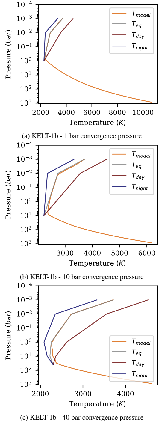
Fig. 3. Equatorially averaged (i.e. the zonal-mean at the equator) T - P profiles (orange) for three models of KELT-1b with different horizontal convergence pressures ( P_{\text{converge}} ), and no radiative forcing, via Newtonian cooling, for P > P_{\text{converge}} . From top to bottom: the convergence pressure of each model is 1 bar, 10 bar, and 40 bar, respectively. In these plots, the equilibrium Newtonian cooling profile is shown in grey, the day-side profile is shown in red, and the night-side profile is shown in blue.
