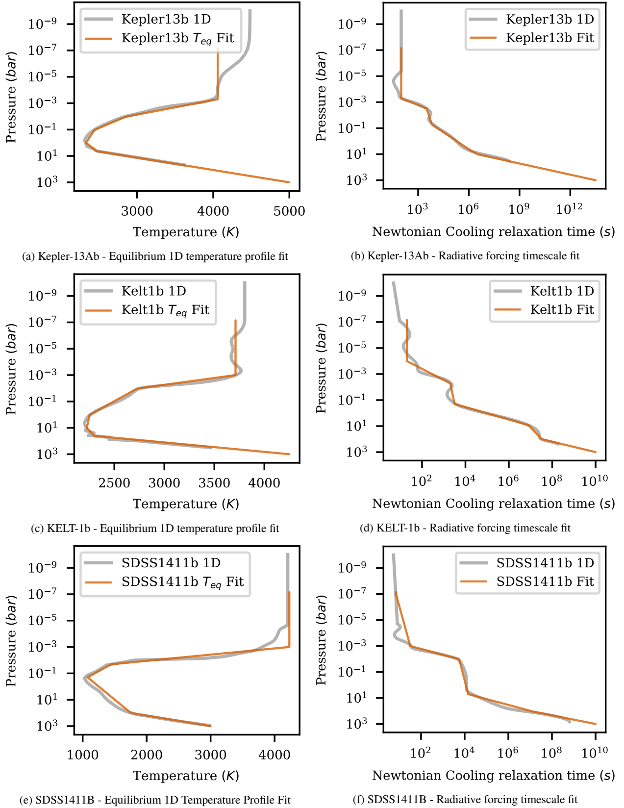
Fig. 2. Fits to the 1D equilibrium temperature-pressure ( T_{eq} – left) and Newtonian cooling relaxation timescale ( \tau_{rad} – right) profiles, which form the basis of the profiles used in our models of Kepler-13Ab (top), KELT-1b (middle), and SDSS1411B (bottom). In all cases, the equilibrium 1D profile is shown in light grey, and the linear in log ( P ) space fit is shown in orange. Note that depending upon the model parameters, including the pressure at which day-night temperature differences go to zero and presence of deep radiative dynamics, these fits may be truncated or modified as required. For full details of the exact fit used in each model, see both Tables 3 and 4.
