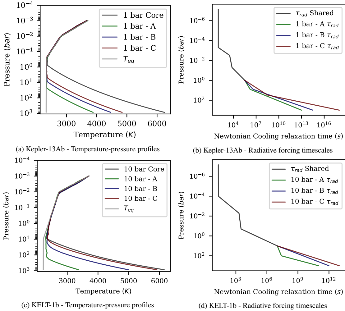
Fig. 7. Snapshots of the T - P profile (left) for a series of test models investigating the effect of deep radiative forcing, via deep isothermal Newtonian cooling, on already evolved (dark grey) models of both Kepler-13Ab (top) and KELT-1b (bottom) with a shallower horizontal convergence pressure. For each brown dwarf, we explore models with increasingly weak deep forcing, as shown by the matching profile on the right (where the full Newtonian cooling timescale profile is found by combining the dark grey profile at lower pressures and the matching coloured profile at higher pressures).
