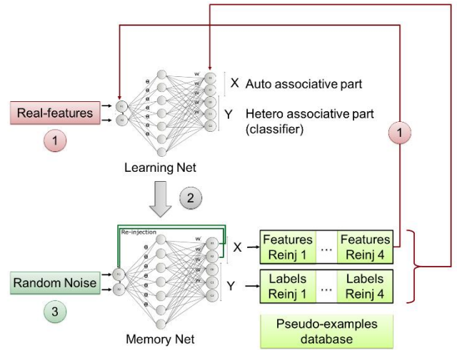
Figure 3: Dream Net model architecture scheme
