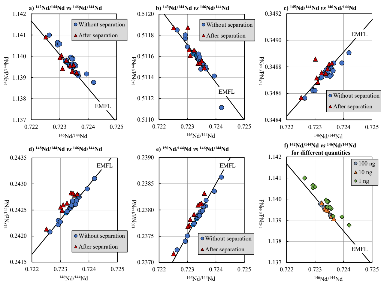
Figure 1: ^X\text{Nd}/^{144}\text{Nd} ( X = 142, 143, 145, 148, 150 ) in comparison to the ^{146}\text{Nd}/^{144}\text{Nd} ratio for the JNdi-1 standard without and after separation (figure a to e, respectively) and ^{142}\text{Nd}/^{144}\text{Nd} vs ^{146}\text{Nd}/^{144}\text{Nd} ratios for different Nd quantities without separation (f). The solid line represents the Exponential Mass Fractionation Law calculated with the Garçon et al. 8 reference values.
