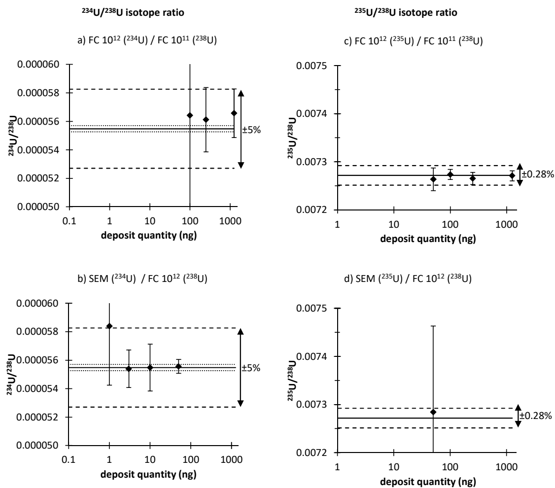
Figure 1: Results for the ^{234}\text{U}/^{238}\text{U} isotope ratio measurements by total evaporation method using Faraday cups coupled to 10^{12}\ \Omega (FC 10^{12} ), 10^{11}\ \Omega current amplifiers (FC 10^{11} ) and the SEM (a and b) and results for the ^{235}\text{U}/^{238}\text{U} isotope ratio measurements by total evaporation method using Faraday cups coupled to 10^{12}\ \Omega , 10^{11}\ \Omega current amplifiers and the SEM (c and d). Each point is represented with a 95% coverage factor uncertainty ( k=2 ). The dark line (-) corresponds to the reference value and the dotted line (...) represents its uncertainty at k = 2 (not represented for better clarity for the isotope ratio ^{235}\text{U}/^{238}\text{U} ): 0.0072718 \pm 0.00000030 for the ^{235}\text{U}/^{238}\text{U} isotope ratio and 0.00005548 \pm 0.00000022 for the ^{234}\text{U}/^{238}\text{U} isotope ratio. The prolonged dotted line (- -) represents the maximal bias fixed by the laboratory.
