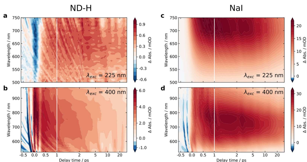
Figure 1 Transient absorption (TA) spectra of aqueous solutions of H-terminated nanodiamonds and NaI solution. a, b, TA signal from ND-H dispersion as a function of probe wavelength and delay time for DUV (a) and visible (b) excitation. c, d, TA signal from NaI as a function of probe wavelength and delay time for DUV (a) and VIS (b)
