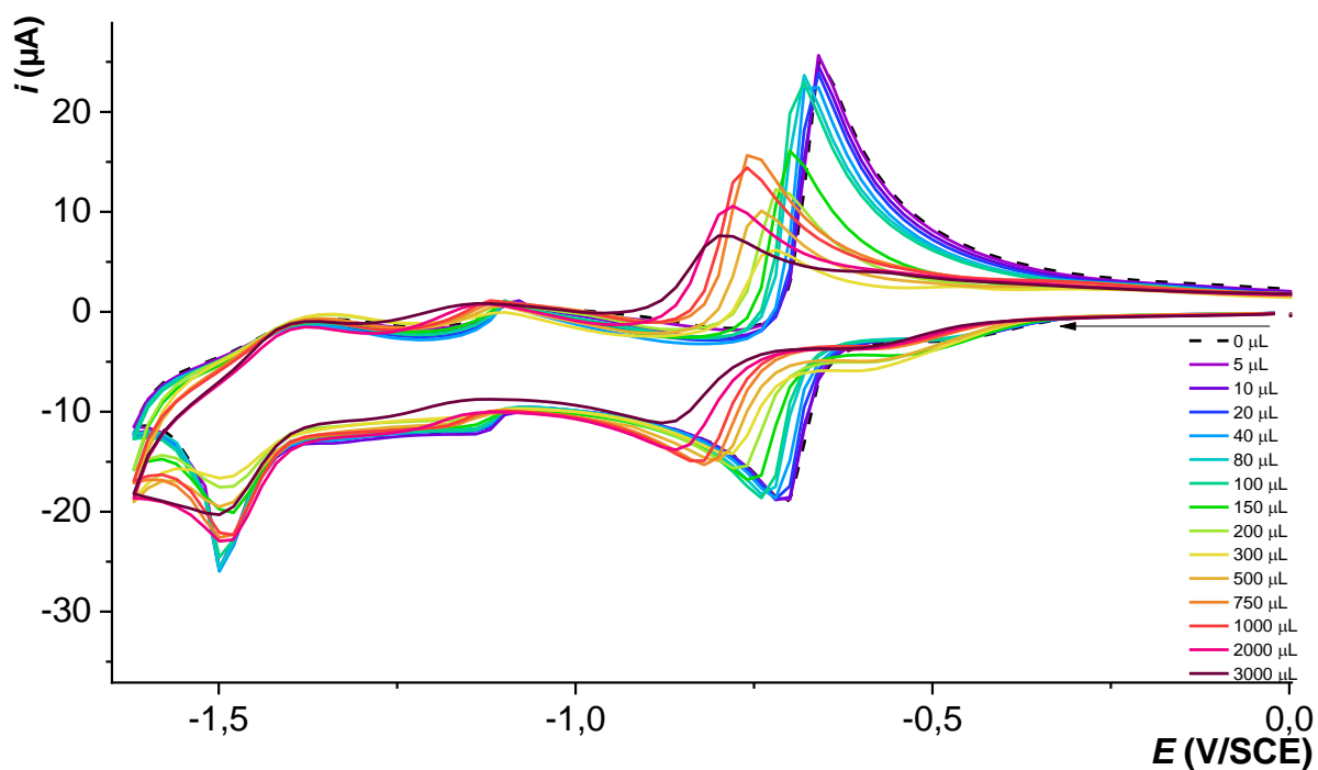
Figure S32. CVs of complex 1 (0.5 mM) under argon in CH 3 CN with increasing amount of DMF with 0.1 M of TBAPF 6 , at 20 °C, CVs are normalized to a concentration of 0.5 mM of complex.
