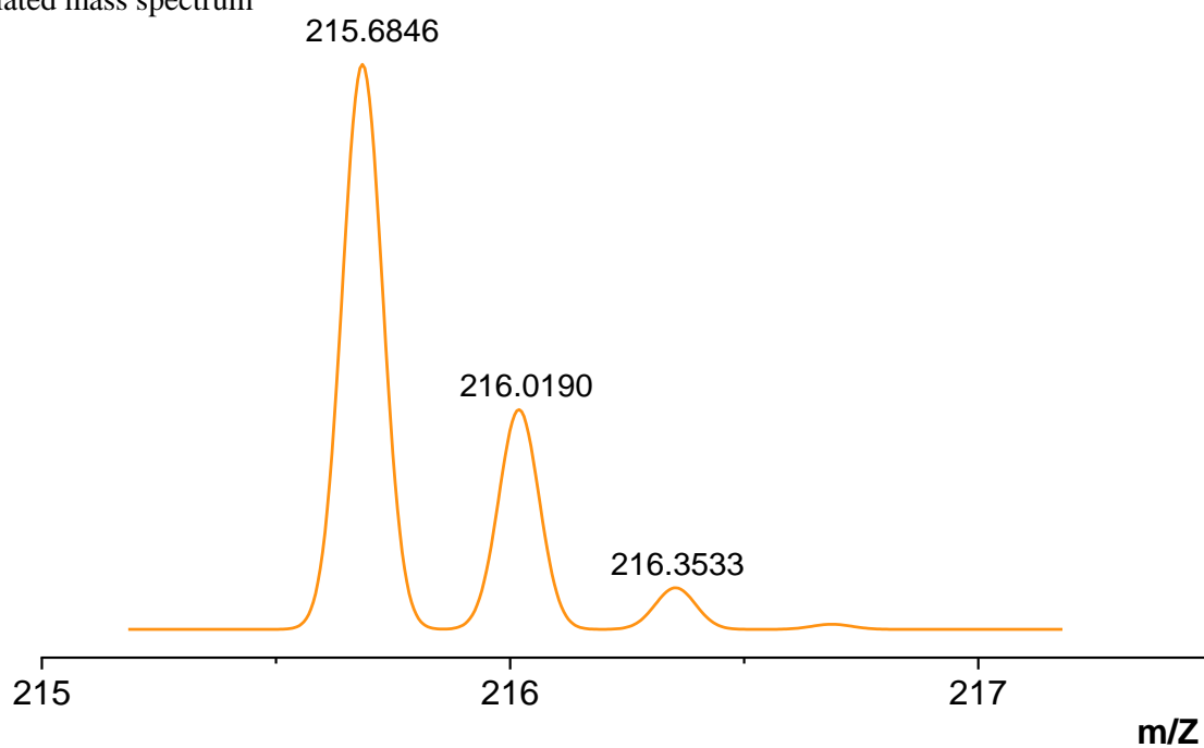
Figure S13. Experimental ESI-MS spectrum of complex 1 in CH 3 OH (top) and simulated ESI-MS spectrum using mMass software (bottom).
