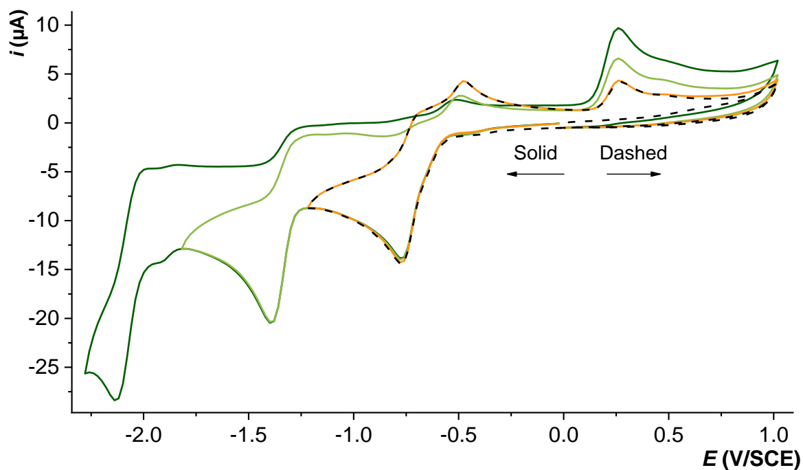
Figure S46. CVs of complex 1 (0.5 mM) under CO in anhydrous DMF with 0.1 M of \text{TBAPF}_6 , scan rate of 0.1 \text{ V}\cdot\text{s}^{-1} .
