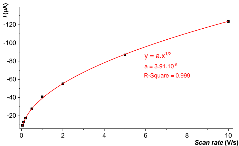
Figure S25. Maximum current ( i_{pf} ) of the cathodic wave R_1 of complex 1 in \text{CH}_3\text{CN} as a function of the scan rate.
