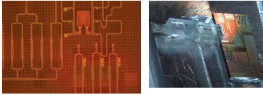
Figure 8 – Top view of PICs manufactured at CEA LETI within EU funded projects PICTURE and COSMICC
