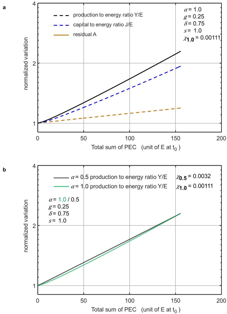
Fig. B2: Production to energy ratio y_\varepsilon = \frac{y}{\varepsilon} , the same ratio for its capital factor j_\varepsilon = \frac{j}{\varepsilon} and the residual A , calculated for \alpha = 1 , according to Eq. (B.13). a: plot on a semilog scale as a function of the total sum of PEC, same abscissa unit (energy) as Fig. B1b. b: comparison of y_\varepsilon = \frac{y}{\varepsilon} on a semilog scale for the two values of \alpha ; both curves are close to a straight line.
