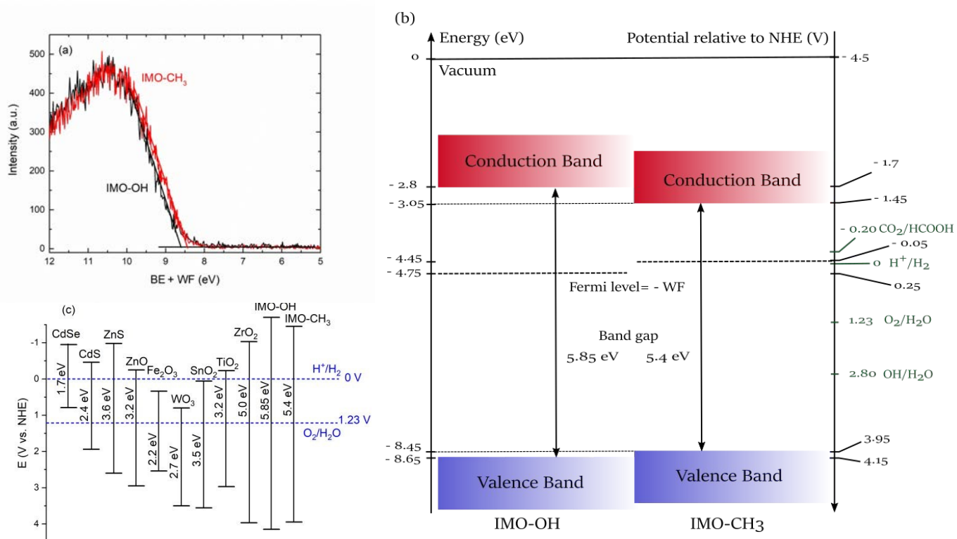
Figure 8. (a) Valence spectra of hydrated IMO-OH (in black) and IMO-CH 3 (in red) measured using synchrotron radiation-based XPS of isolated nanotubes at 100 eV photon energy. The spectra are normalized with respect to the top of the valence band. The zero energy corresponds to the vacuum level. The linear fits enable measuring the energy of the top of the valence bands. (b) Schematics of the band diagrams of IMO-OH and IMO-CH 3 . The various energies are given in absolute (eV) and also in relative (in V vs. NHE) potential scale. The band edges of imogolites are also represented relative to the reversible oxidation and reduction potential of water (at pH = 0). (c) Band edges of selected compounds. The values of the band edges are taken from reference 57 .
