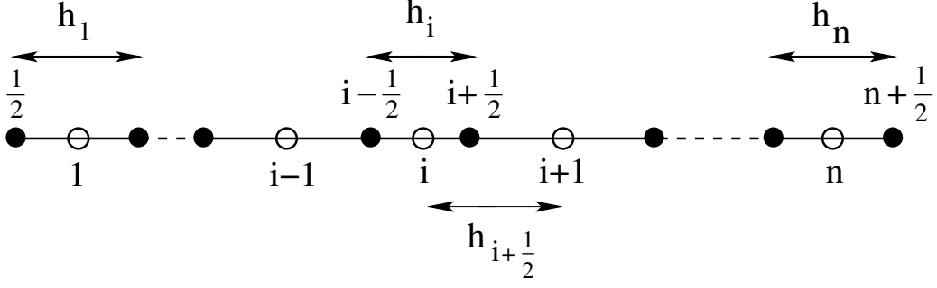
Figure 1: Definition of the mesh: x_i are cell centers, x_{i+\frac{1}{2}} are nodes.
