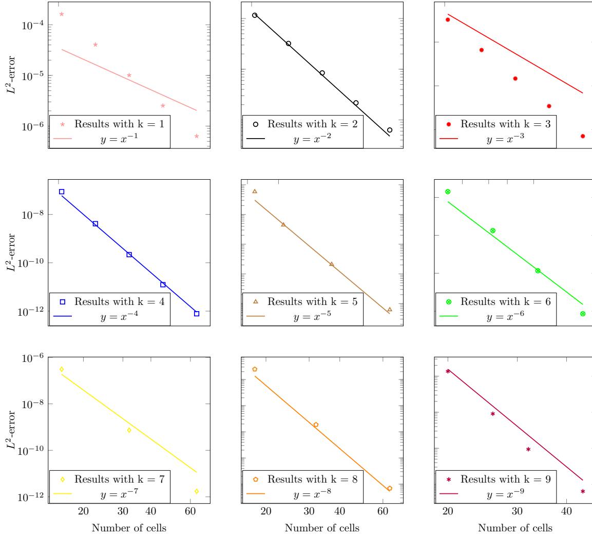
FIGURE 10. L^2 -error with symmetric scheme and discontinuous right hand size for problem of Sec. 4.4.
