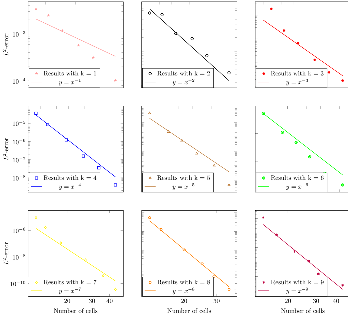
FIGURE 8. L^2 -error with symmetric scheme and random mesh for problem of Sec. 4.2.
