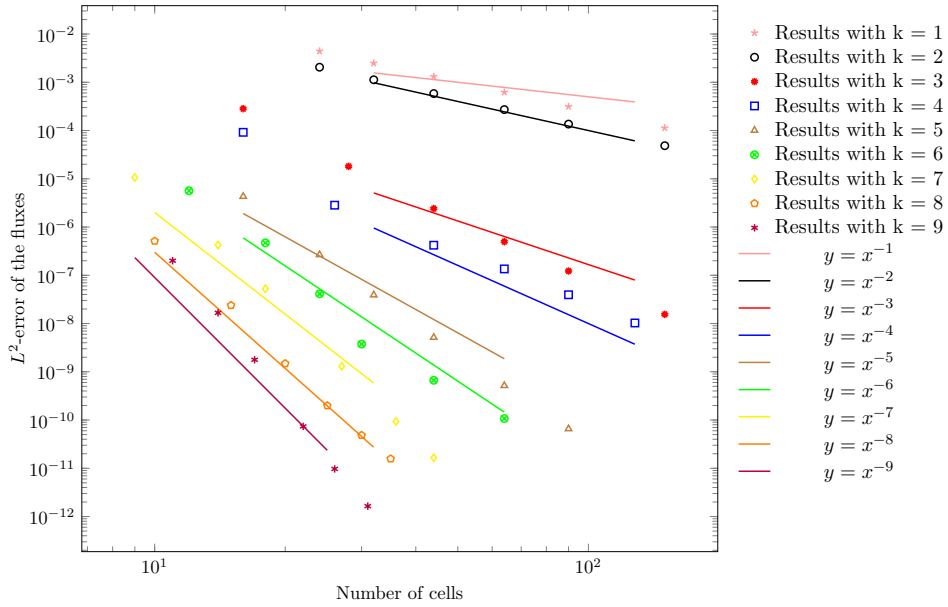
FIGURE 5. L^2 -error of the fluxes with the symmetric scheme for problem of Sec. 4.2.
