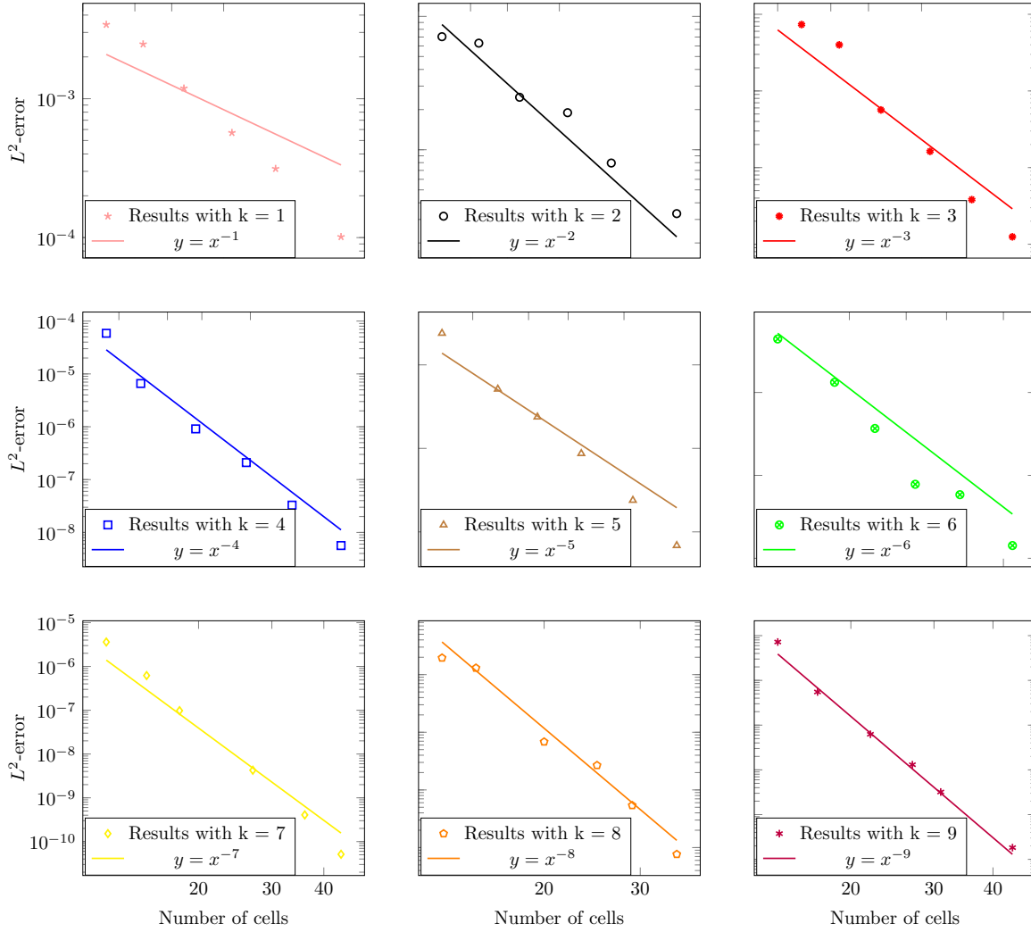
FIGURE 6. L^2 -error with non-symmetric scheme and random mesh for problem of Sec. 4.2.
