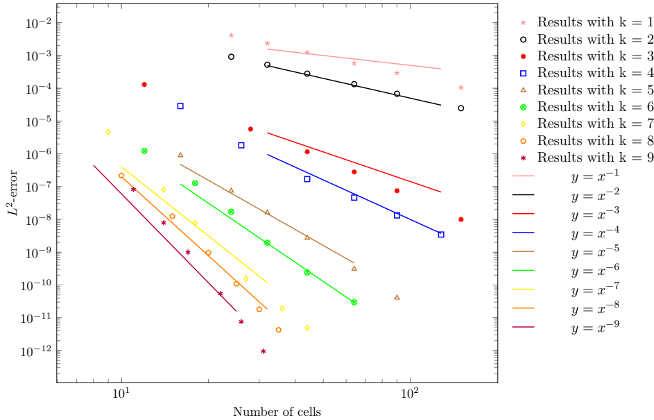
FIGURE 4. L^2 -error with the symmetric scheme for problem of Sec. 4.2.
