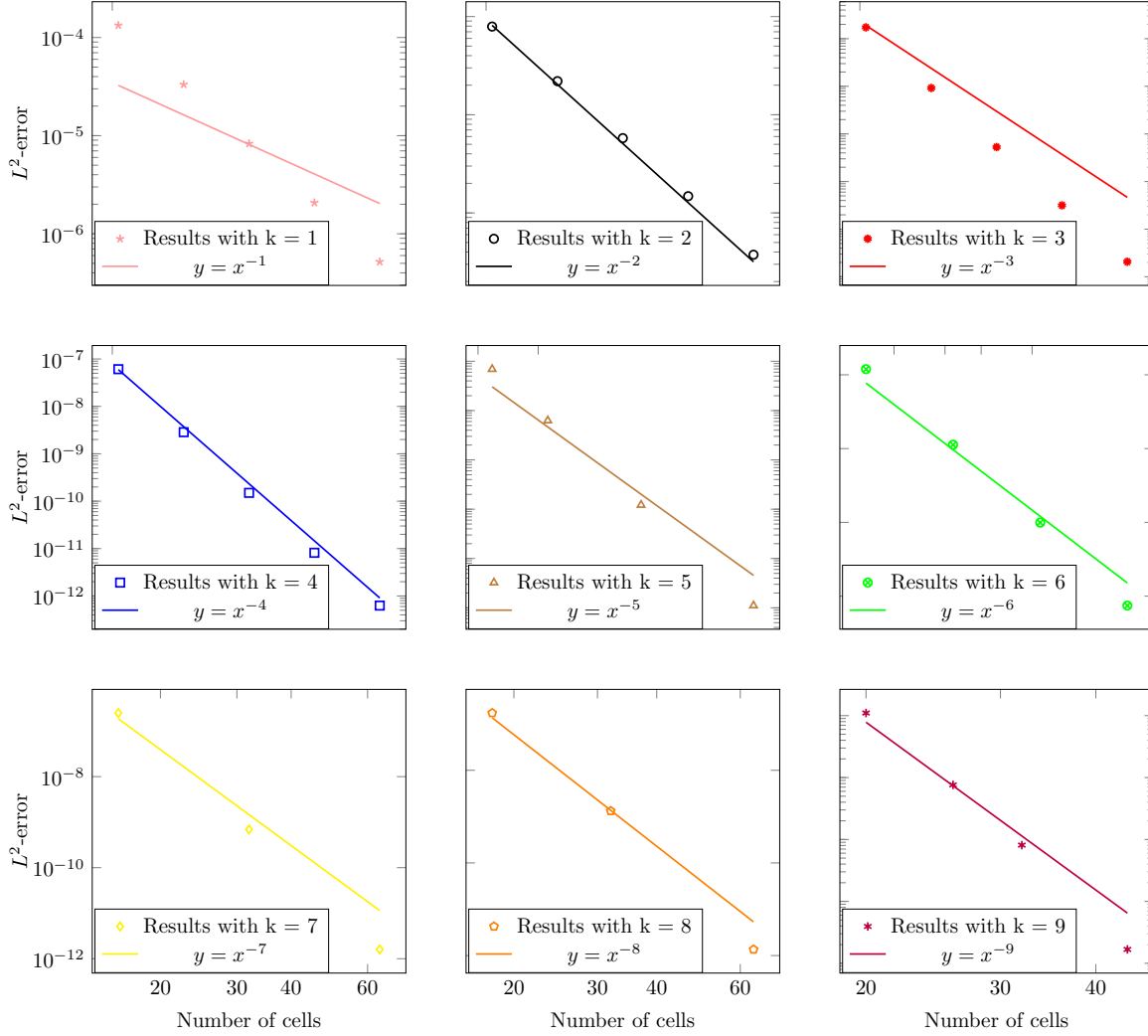
FIGURE 11. L^2 -error with symmetric scheme and discontinuous \kappa for problem of Sec. 4.5.
