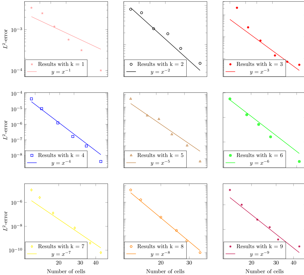
FIGURE 9. L^2 -error on the fluxes with the symmetric scheme and random mesh for problem of Sec. 4.2.
