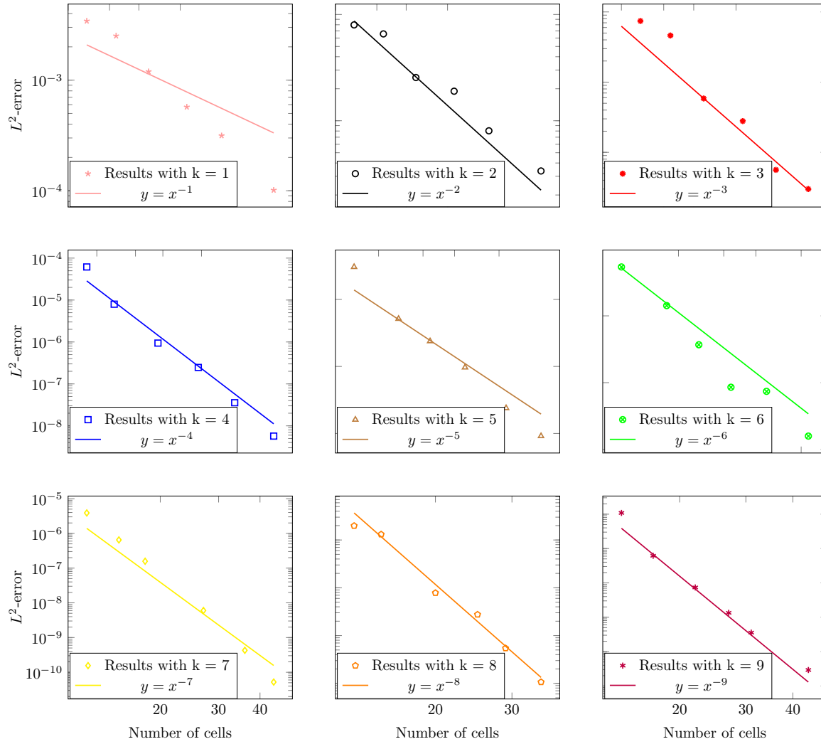
FIGURE 7. L^2 -error on the fluxes with non-symmetric scheme and random mesh for problem of Sec. 4.2.
