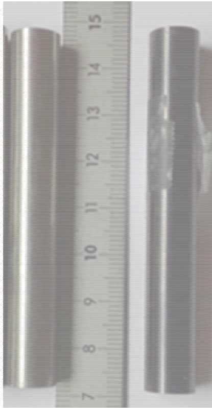
Photo of Zy4 claddings. Some Zy4 claddings were artificially oxidized.
