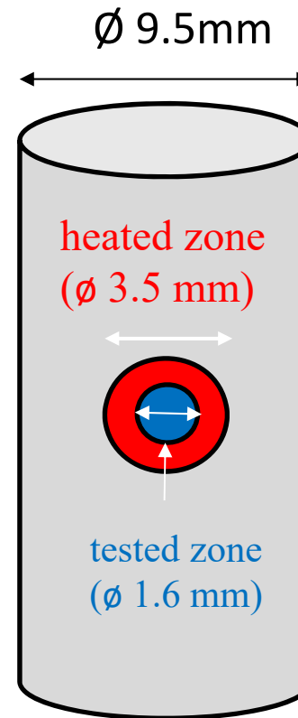
Schematic comparison of the Zy4 cladding diameter and those of the heated zone (in red) and of the tested zone on it (in blue).
