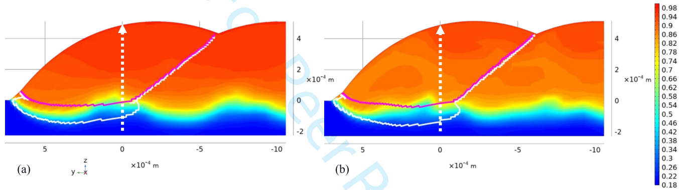
Figure 5. (a) Turbulent and (b) laminar model results, cross-section ( yz cut plane at x = -1 mm) after solidification of the Cr mass fraction color mapping with the contours of the molten zone, chromium liquidus (in magenta) and local liquidus (in white), projected along x . White dashed arrow: see figure 10.
