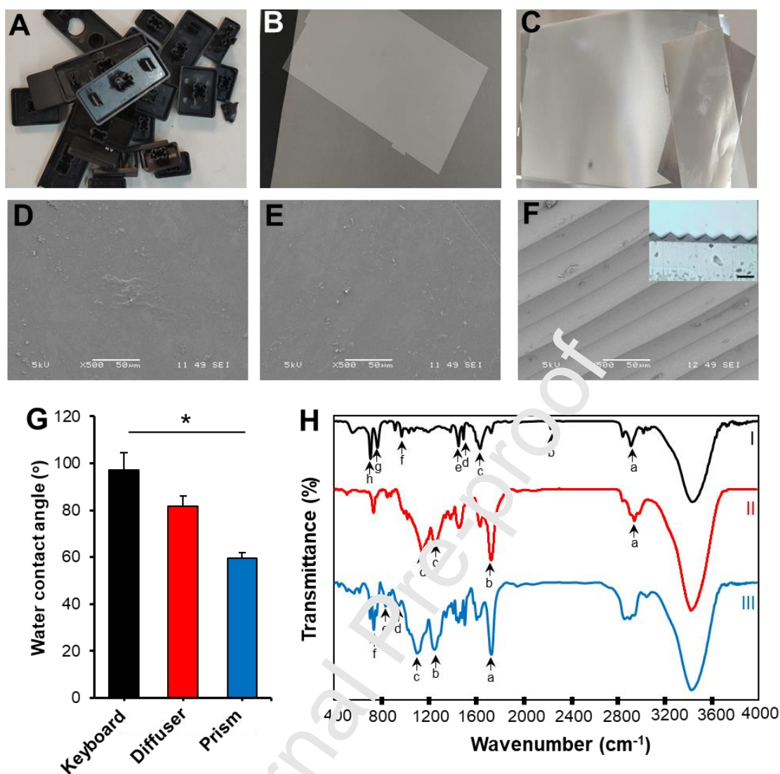
Figure 1. Representative photographs (A-C) and SEM images (D-F) of the keyboard, diffuser sheet, and prism sheet were employed in this study. (Insert: cross-section of prism sheet, scale bar: 50 \mu m). (G) Static water contact angle measurements of the E-plastics. (H) FTIR spectra of the keyboard (I), diffuser (II), and prism sheet (III).
