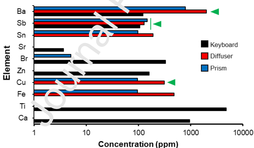
Figure 2. XRF analysis of E-plastics. Green arrow indicates elements that are detected at levels that exceeds the restriction limits of hazardous substances in accordance to 2009/48/EC, 2011/65/EU and 94/62/EC. Threshold limits of various metal species: Cu (156ppm), Zn (938ppm), As (3.8ppm), Sr (1125ppm), Sn (3750ppm), Sb (45ppm), Ba (1125ppm), Pb (13.5ppm).
