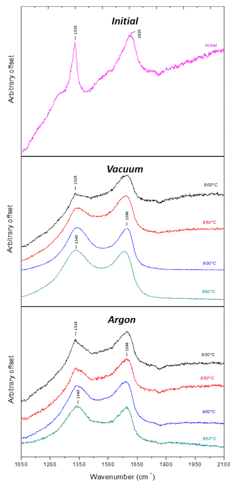
Figure 3. Raman spectra of initial and annealed DND from 800 °C to 950 °C for both atmospheres. The excitation wavelength was 532 nm.
