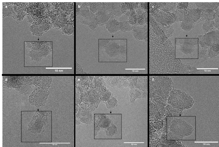
Figure 5. HR-TEM images of DND: a ), b ), and c ) initial particles; d ) 800 °C 4h; e ) and f ) 950 °C 4h. Images recorded near to Scherzer defocus are provided into insets.
