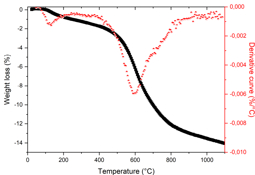
Figure 1. TGA spectra of initial DND annealed under argon atmosphere (black) and TGA derivative curve (red).
