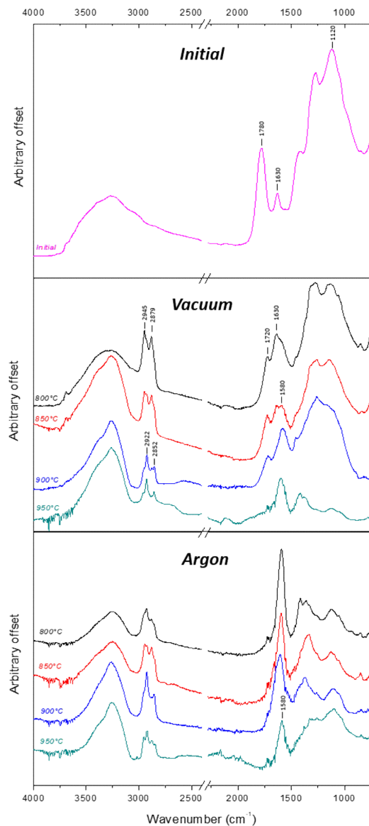
Figure 2. FTIR spectra of initial and annealed DND from 800 °C to 950 °C for both atmospheres.
