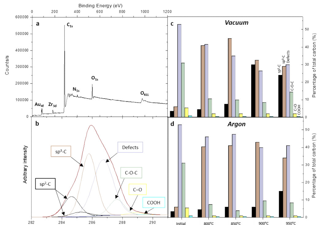
Figure 4. a) Wide XPS spectrum; b) typical C1s core level spectrum with fitting: DND after annealing at 950 °C under argon atmosphere; evolution of the six different components at C1s for initial and DND annealed under c) vacuum and d) argon atmospheres.
