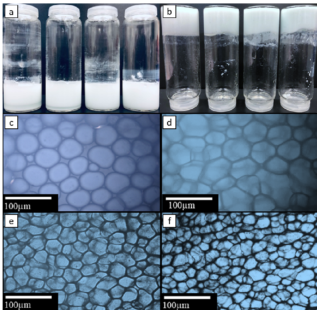
Fig.1. (a) Pickering emulsions with 2.5 wt.% MIL-96(Al) and different paraffin volume ratios: from left to right, \phi_v = 0.5, 0.6, 0.7 and 0.8 . (b) Pickering emulsions with \phi_v = 0.8 and different concentrations of MIL-96(Al): from left to right, W_{MOF} = 1, 2, 3.5 and 5 wt.%. Optical micrographs of emulsions with 5 wt.% MIL-96(Al) and paraffin volume ratios of (c) 0.5 , (d) 0.6 , (e) 0.7 , and (f) 0.8 .
