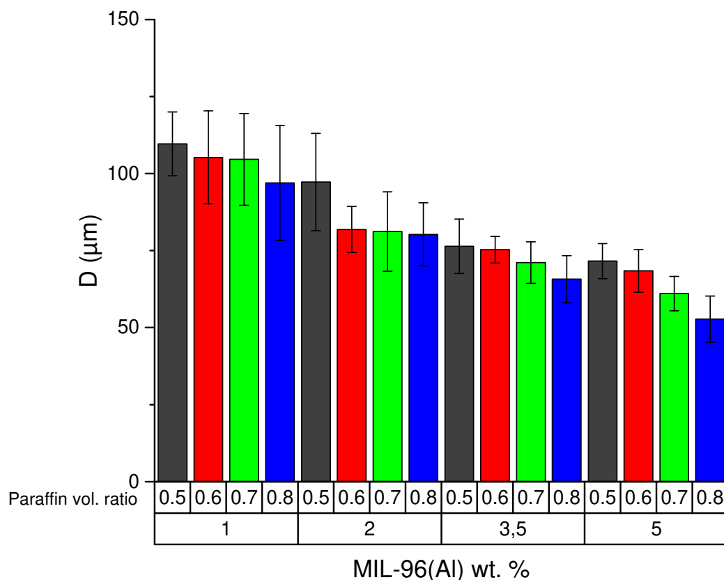
Fig. 2. Mean droplet sizes ( D ) in paraffin-in-water emulsions stabilized by MIL-96(Al) as a function of the paraffin volume ratio and the MIL-96(Al) concentration. The error bars represent standard deviations.
