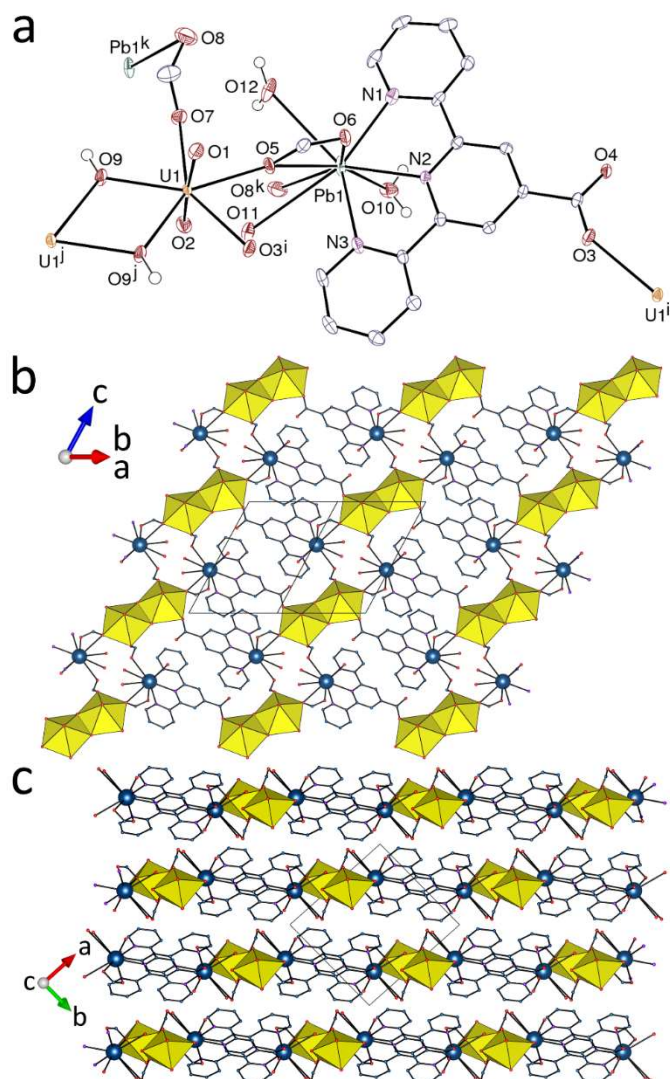
Fig. 2 (a) View of compound 2 with displacement ellipsoids shown at the 50% probability level and carbon-bound hydrogen atoms omitted. Symmetry codes: i = -x, 1 - y, 2 - z ; j = 1 - x, 2 - y, 2 - z ; k = 1 - x, 2 - y, 1 - z . View of the dimeric assembly with uranium coordination polyhedra yellow and lead atoms shown as blue spheres. (c) Packing with layers viewed edge-on.
