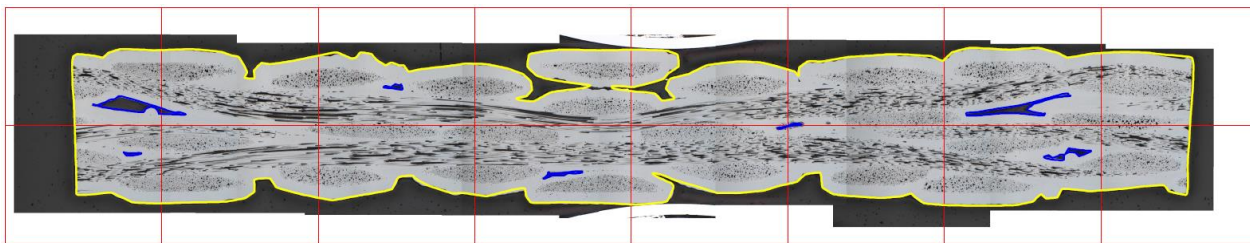
Figure 2. Polished section of a composite processed by the MICROVISION Instrument™ Areas software. The section is delimited in yellow and the porosities are indicated in blue.
