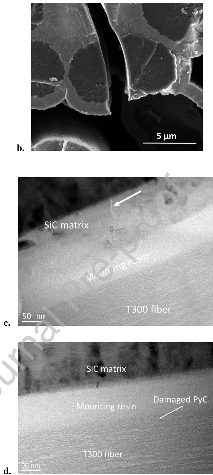
Figure 9. Fracture surface of T300/PyC/SiC composite by SEM (a. and b.) and TEM cross-section of the F/M interface of T300H/SiC (c.) and T300/PyC/SiC (d.) composites after tensile tests.
