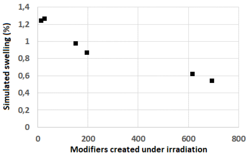
Figure 15: Swelling as a function of the number of modifiers formed under irradiation.
