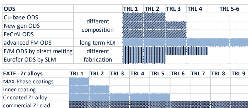
Fig. 4. In-depth look at specific categories: a) selected projects on ODS alloys and b) EATF (Zr alloys) [Data and graphs presented in this paper are only based on outputs of the survey carried out within the EGISM. They do not reflect all activities performed in OECD countries.]
