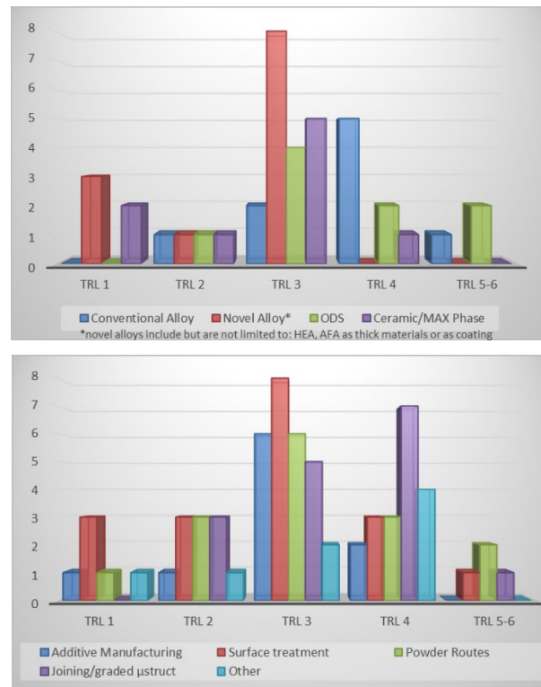
Fig. 3. Number of projects reaching the specified TRL (a) by materials family; (b) by process category [Data and graphs presented in this paper are only based on outputs of the survey carried out within the EGISM. They do not reflect all activities performed in OECD countries.]
