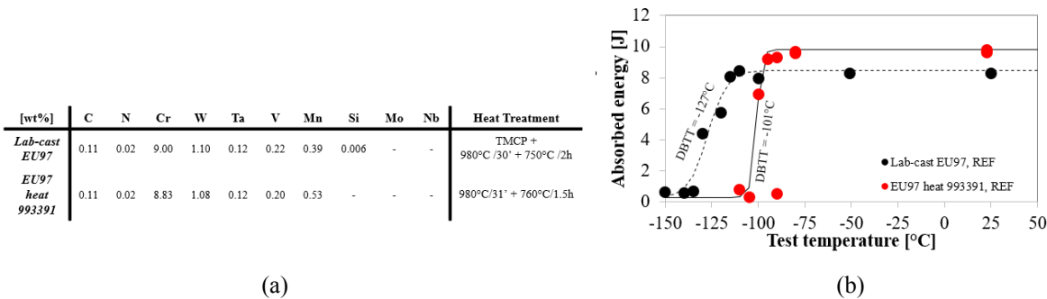
Fig. 7. Comparison of the reference E97 (grade 2, heat 993391) and optimized lab-casted E97 fabricated by OCAS. The main difference comes in the additional hot rolling step applied at 850°C, which generates some improvement in DBTT, a different initial precipitation state, somewhat lower strength at RT which however becomes comparable to that of ref. E97 at higher temperature. The figure summarizes chemical composition (a) and absorbed energy vs. test temperature (b)
