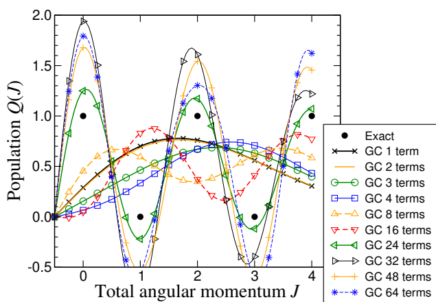
(a) Exact and Gram-Charlier-like approximation for the total angular momentum distribution Q(J) .
