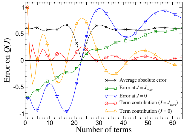
(b) Error done using the Gram-Charlier-like approximation for the total angular momentum distribution Q(J) . The abscissa is the number of terms kept in the expansion (III.2a). The contribution of each term to the sum, normalized to the first term, is also shown.
