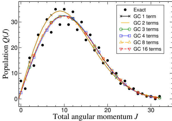
(a) Configuration j_1 = 15/2, N_1 = 8
