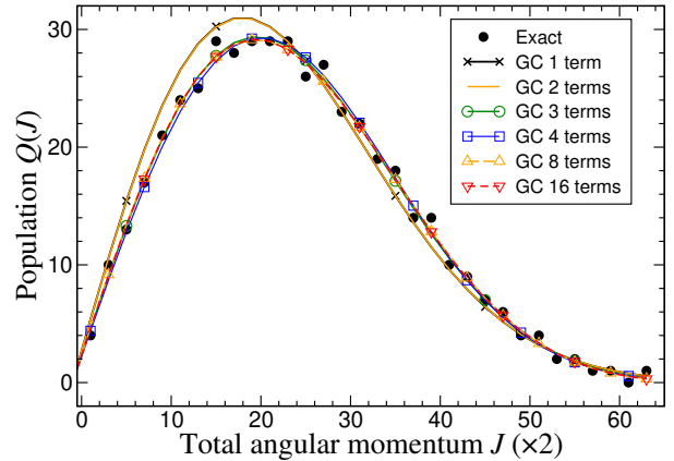
(b) Configuration j_1 = 15/2, N_1 = 7
