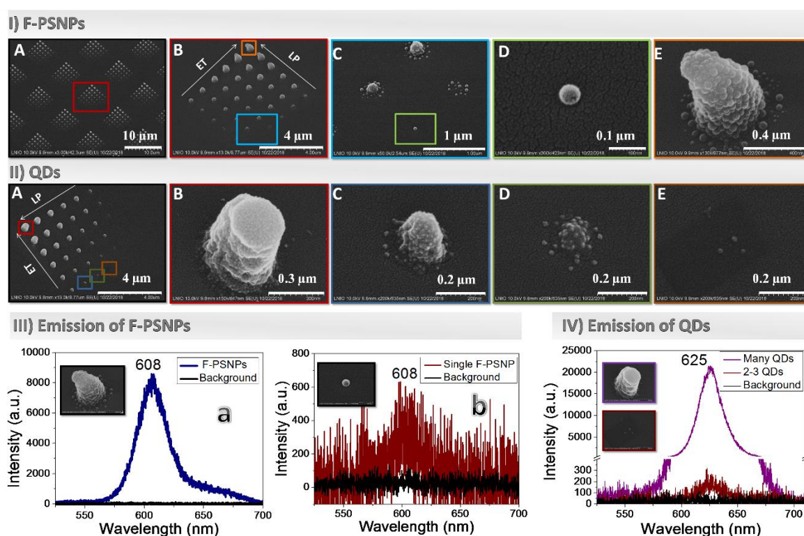
Figure 8. I) SEM images of patterns containing functionalized polymer dots after immersion in Fluorescent PSNPs (size \sim 50 nm) (A), magnification on one pattern corresponding to polymer dots obtained at different ET and LP (B), magnification on B (C, D and E). II) SEM image of one pattern of functionalized polymer dots, obtained at different ET and LP, after immersion in CdSe/ZnS red-emitting QDs (A) magnification on A (B, C, D and E). III) Emission spectra of many fluorescent PSNPs attached on a polymer microdot excited by a blue laser (LP 2 \mu\text{W} / 1 second) (a) and a single fluorescent PSNP attached on a very small polymer
