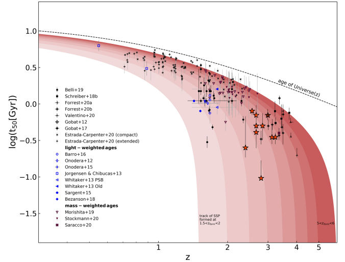
Fig. 16. Stellar ages as a function of observed redshift of \log(M_*/M_\odot) > 10.5 quiescent galaxies. Adapted from Onodera et al. (2015). Here mass-weighted ages from the literature differ from t_{50} in that they do not specifically refer to the lookback time at which 50% of M_* is formed. The four targets selected from Schreiber et al. (2018) correspond to those recently followed up by Esdaile et al. (2021). Solid grey lines show, from thin to thick, the age of simple stellar populations made at a z_{\text{form}} from 1.5 to 5. The dotted red line marks the age of the Universe as a function of redshift.
