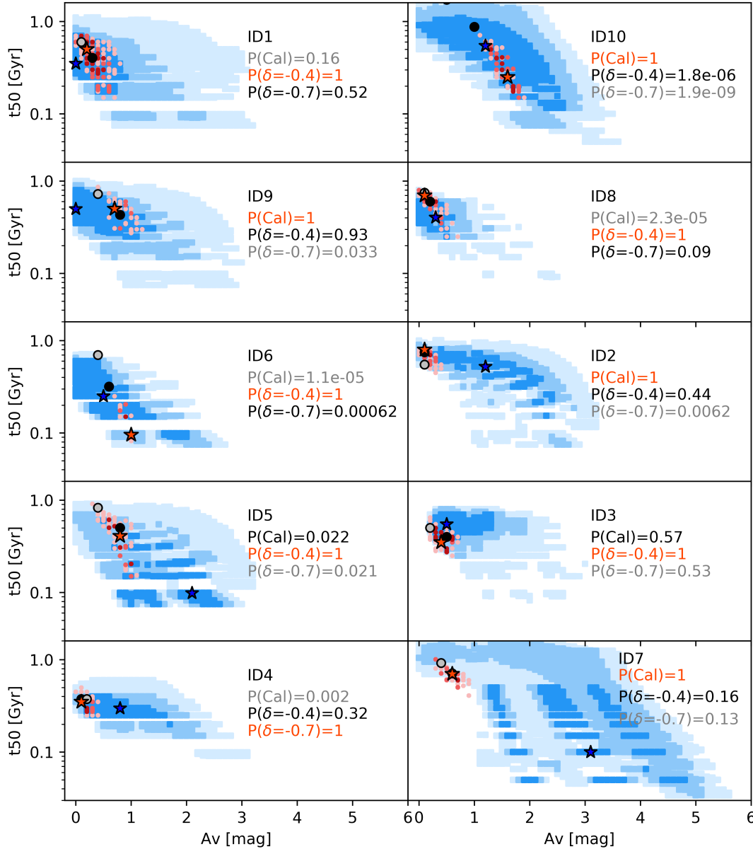
Fig. 10. Mass-weighted ages and dust extinction values for our targets. Blue squares mark the confidence regions ( 3 to 1 \sigma going from light to dark points) extracted from the spectra alone. Red points show the solutions of the combined fit. Blue and red stars in each panel mark the best-fit solution from the spectroscopic fit and the combined fit, respectively. The relative probabilities of the extinction laws are shown for each galaxy. As a reference, we report the best-fitting combined solution at fixed extinction law as black and grey dots. Their colour-coding follows that of the aforementioned relative probabilities.
