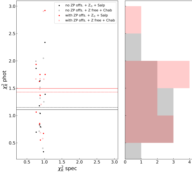
Fig. 5. Distributions of photometric reduced \chi^2 before (red dots) and after removing the ZPs re-calibration (black dots). Median values are marked with solid red and black lines. \chi^2_R values obtained adopting a Chabrier IMF and leaving the metallicity free to vary are shown as empty squares. Their corresponding medians are shown as dashed lines.
