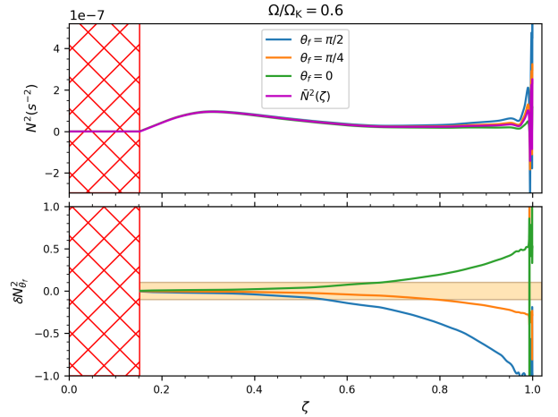
Fig. 4. Profile of the squared Brunt-Väisälä frequency N^2 and the relative error \delta N_{\theta_f}^2 of the adopted approximation (Eq. (42)) as a function of \zeta at different colatitudes \theta_f using an ESTER model rotating at 60% of the Keplerian breakup rotation rate (The light orange area indicates the margin of error which we allow and the red hatched area represents the convective region of the star).
