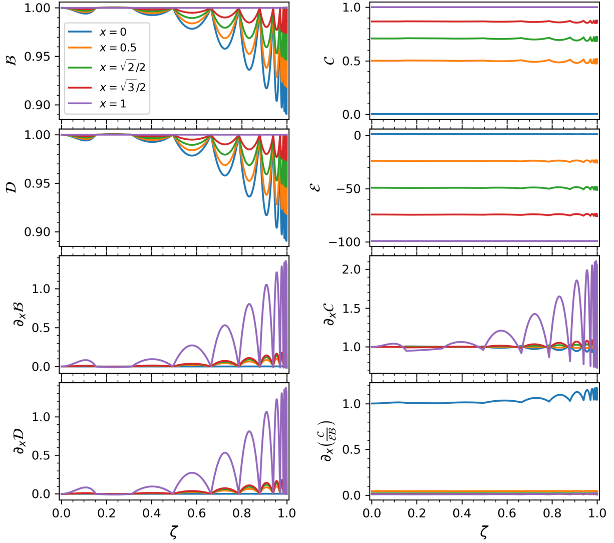
Fig. B.1. Profiles of the coefficients \mathcal{B} , \mathcal{C} , \mathcal{D} , \mathcal{E} , \partial_x \mathcal{B} , \partial_x \mathcal{C} , \partial_x \mathcal{D} and \partial_x \left(\frac{\mathcal{C}}{\mathcal{E}\mathcal{B}}\right) involved in the derivation of the GLTE (Eq. (34)) as a function of \zeta at different reduced colatitudes x using an ESTER model ( M = 3M_\odot , X_c = 0.7 ) rotating at 20% of the Keplerian break-up rotation rate for a spin parameter \nu = 10 .
