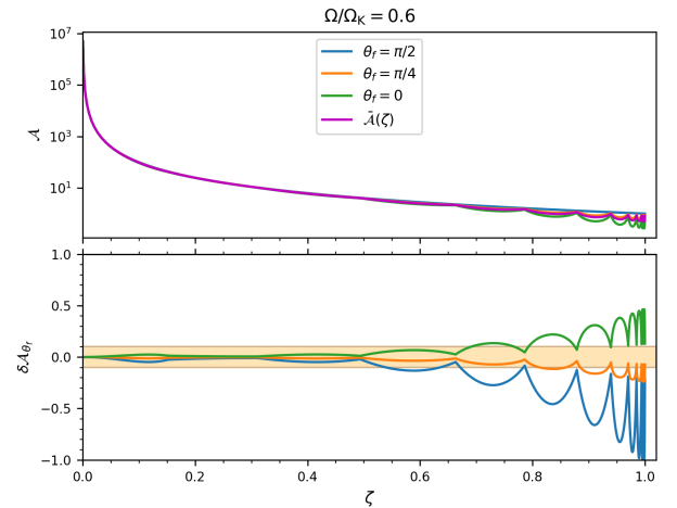
Fig. 5. Profile of the coefficient \mathcal{A} and the relative error \delta \mathcal{A}_{\theta_f} of the adopted approximation (Eq. (43)) as a function of \zeta at different colatitudes \theta_f using an ESTER model rotating at 60% of the Keplerian breakup rotation rate (The light orange area indicates the margin of error which we allow).
