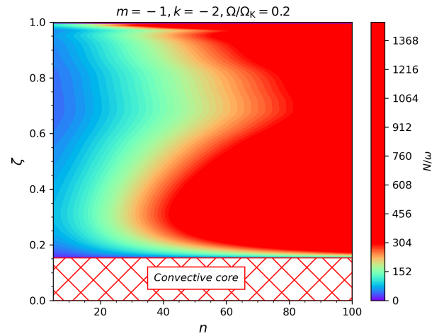
Fig. 13. N/\omega term as a function of the pseudo-radius \zeta and the radial order n for \{k = 0, m = 1\} (top panel) and \{k = -2, m = -1\} (bottom panel) modes at \Omega/\Omega_K = 20\% .
