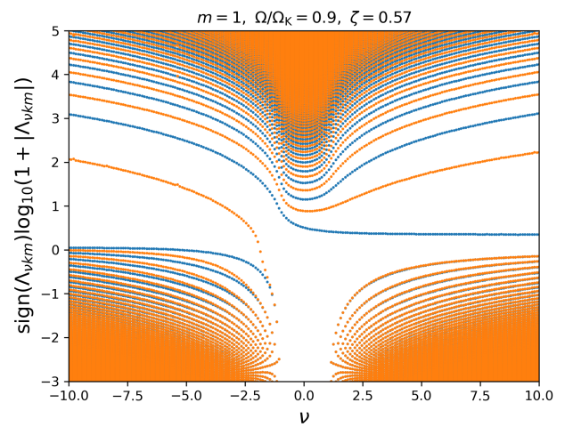
Fig. 7. Spectrum of the GLTE as a function of the spin parameter \nu at \zeta = \zeta_{\text{limit}} and m = 1 for \Omega = 0.2\Omega_K (above) and \Omega = 0.9\Omega_K (below). Blue (respectively, orange) dots correspond to even (respectively, odd) eigenfunctions.
