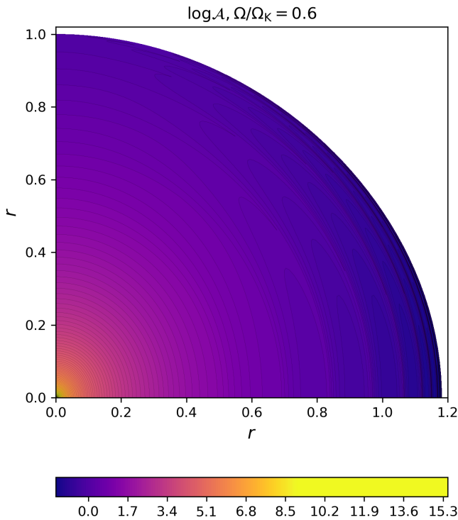
Fig. 3. Coefficient \mathcal{A}(\zeta, \theta) profile for \Omega/\Omega_K = 60\% .
