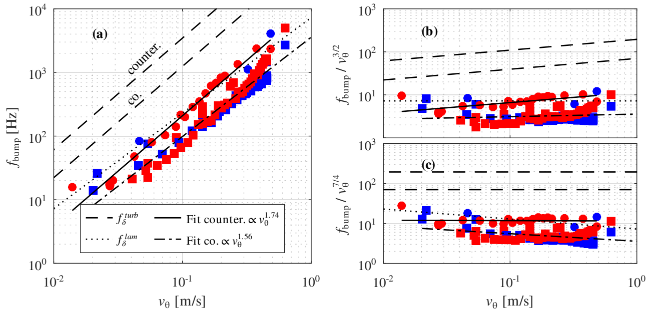
FIG. 7. Representative frequency of the spectral bump f_{\text{bump}} as a function of the azimuthal velocity v_{\theta} in counter-rotation (square symbols) and co-rotation (round symbols) at 2 K (red) and 1.6 K (blue). The solid and dash-dotted black lines show the best fit of the form f_{\text{bump}} \propto v_{\theta}^{\gamma} for the counter-rotating and co-rotating cases respectively. The dashed lines correspond to f_{\delta}^{\text{turb}} computed from eq. (7) for both kinds of flows, while the dotted line corresponds to f_{\delta}^{\text{lam}} , eq. (5). (a): raw frequency. (b): frequency divided by v_{\theta}^{3/2} . (c): frequency divided by v_{\theta}^{7/4} .
