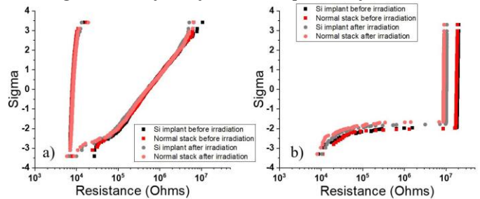
Fig. 4: LRS and HRS (a) and Pristine resistance (b) normal distribution results on two memory stacks (pure HfO 2 and Si-implanted HfO 2 ) after irradiation at low fluence ( 10^9 ions/cm 2 ) and with no-irradiation.
