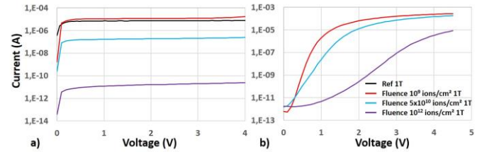
Fig. 3: Measurements carried out on single NMOS transistors (Width=660nm and Length=500nm). a) I_d(V_d) at V_g=1.3 V after irradiation at three various fluences ( 10^9 ions/cm 2 , 5 \times 10^{10} ions/cm 2 , 10^{12} ions/cm 2 ) and with no irradiation (reference). b) I_d(V_g) at V_d=1.3 V after irradiation (three fluences).
