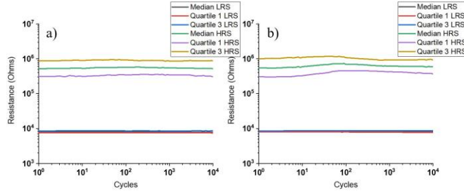
Fig. 5: 10k Cycles endurance succeeded on HfO 2 stack (a) and Si implanted HfO 2 -s stack (b) on 3072 devices after irradiation at a fluence of 10^9 ions/cm 2 .
