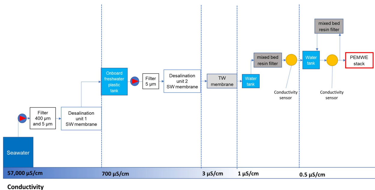
Figure 2. Schematic of the seawater purification system from seawater down to deionised water used to feed the PEMWE. An approximative conductivity value is presented for each step of the processes.
