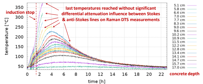
Figure 6 – OFS cables temperature vs. time during VULCANO experiment (Raman DTS reflectometry)
