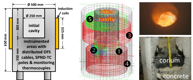
Figure 5 – VULCANO concrete crucible with OFS cables arrangement and thermite ignition
