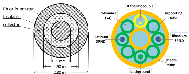
Figure 3 – Left: SPND structure with Rh or Pt emitter – Right: instrumented SPNDs-TC pole structure
