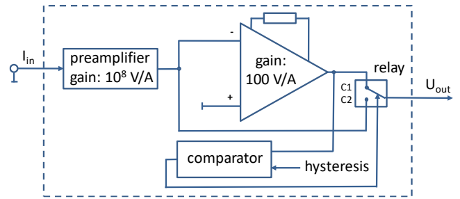
Figure 2 – Low currents & wide range [1 pA, 100 nA] amplification device for SPND current measurements
