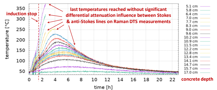
Figure 6 – OFS cables temperature vs. time during VULCANO experiment (Raman DTS reflectometry)
