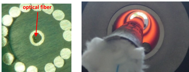
Figure 4 – Left : strain sensor cable section – Right : sustainability to temperature qualification test
