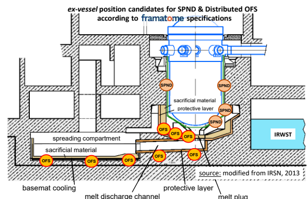
Figure 1 – SPNDs-TC & OFS cables ex-vessel position candidates for Severe Accident monitoring (e.g.: EPR)
