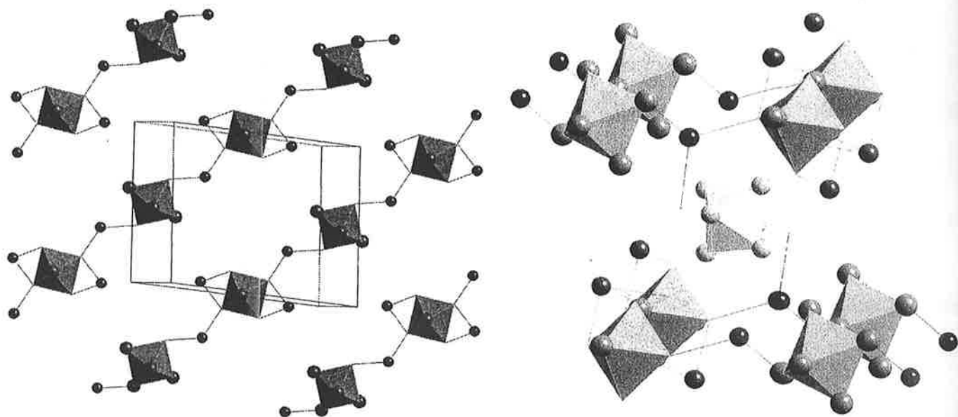
Fig 10. Polyhedral representation of the chains of [\text{Mg}(\text{H}_2\text{O})_6]^{2+} cations linked by hydrogen-bonded water molecules (left) and the cage encapsulating the \text{Re}_6\text{S}_6\text{Cl}_8^- cluster anion (right).
