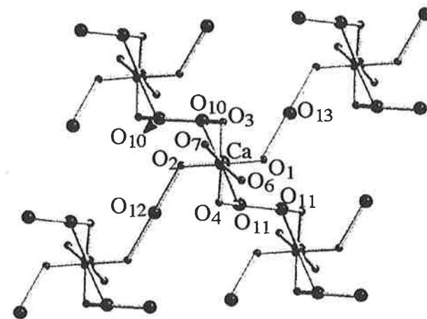
Fig 4. Two orthogonal views, normal (top) and along (bottom) the Ca-O5 direction of the first hydration shells of [\text{Ca}(\text{H}_2\text{O})_7]^{2+} ions in 6 and their connecting pattern. Selected bond lengths (Å): Ca-O1, 2.431; Ca-O2, 2.382; Ca-O3, 2.487; Ca-O4, 2.391; Ca-O5, 2.408; Ca-O6, 2.438; Ca-O7, 2.540; O1...O13, 3.177; O2...O12, 3.213; O3...O10, 2.981; O4...O11, 2.945; O5...O10, 2.845; O5...O11, 2.789.
