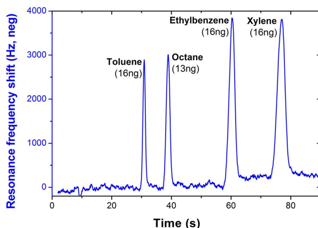
Figure 11. Chromatogram (raw data) measured by a crossbeam NEMS coated with the same adsorbent layer as in Fig.10. The NEMS (at room temperature) is placed behind a standard 2m long capillary column (at 50°C). Brackets indicate the amount of each analyte injected into the GC column. Peak maxima are larger and shorter than in Fig.10, the analysis time is divided by two.
