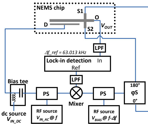
Figure 4. Heterodyne piezoresistive downmixing scheme (with one single actuation electrode) for integrated electromechanical transduction of the crossbeam mechanical motion. PS stands for power splitter, LPF for low-pass filter and \phi S for phase shifter.
