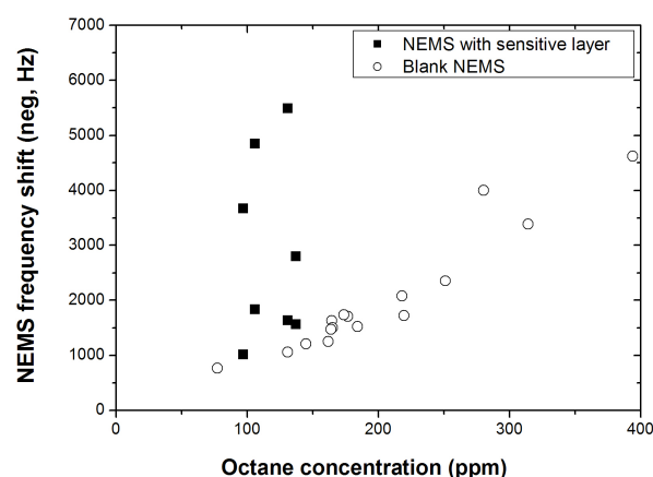
Figure 9. Example of response curves for octane: the frequency shift is plotted as a function of the concentration for several NEMS with different coating layers.
