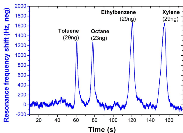
Figure 10. Chromatogram (raw data) measured by a crossbeam NEMS coated with the adsorbent layer selected after the experiments of Fig. 8 and 9. The NEMS is placed behind a miniaturized 1m long silicon \mu GC coated with PDMS (Fig.1), both elements are at 50°C. Brackets indicate the amount of each analyte injected into the GC column.
