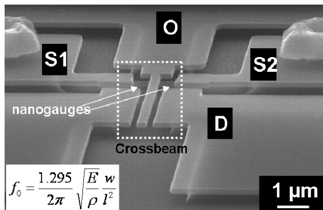
Figure 2. SEM image of a released, single-crystal silicon NEMS resonator: a so-called 'crossbeam' with its four actuation/detection ports. The bias voltages are applied on the lateral nanogauges through S1 and S2, the actuation voltages through D and the output signal V_{OUT} is measured on O. The beam dimensions are: 3.2μm long ( l ), 300nm wide ( w ), 160nm thick. The gauges width is 80nm. The inset indicates the equation of the resonance frequency f_0 of the first in-plane flexural mode ( E and \rho stand for the Si Young's modulus and density).
