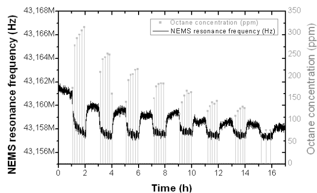
Figure 8. Gas sensing response (resonance frequency shift) at equilibrium of a blank NEMS resonator (without functionalization layer) to various concentrations of octane.
