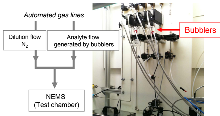
Figure 7. Gas test bench for measurements at equilibrium. Bubblers are used to generate gaseous analytes from liquid or solid origin. The concentration delivered by the bubbler as well as the flow rate, pressure, temperature and relative humidity are recorded in real time
