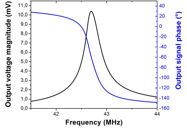
Figure 5. Open-loop frequency response measured at ambient pressure for V_{IN\_AC} =2V peak-to-peak, V_{IN\_DC} =10V, and V_{BIAS} =2V pp. The quality factor is 165 for a resonance frequency of 42.75MHz.
