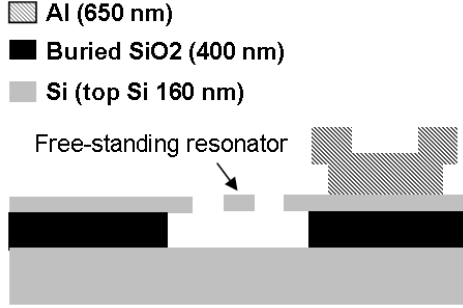
Figure 3. Simplified cross-section of the NEMS resonator and its leads (at the end of the technological process).
