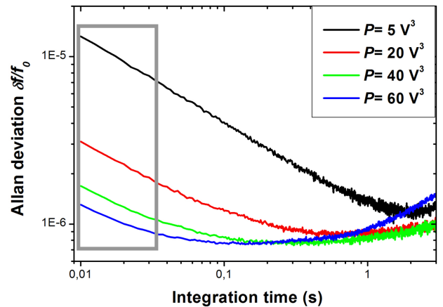
Figure 6. Allan deviation \delta f / f_0 of a crossbeam measured at ambient pressure for various products P = [V_{IN\_AC} \times V_{IN\_DC} \times V_{BIAS}] \text{ [V}^3\text{]} (the output signal is proportional to P ). In the grey region, the higher is P , the better is the resonator frequency noise as expected from [7].
