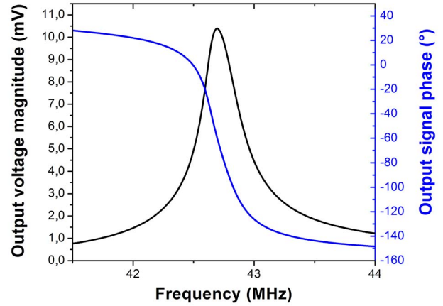
Figure 5. Open-loop frequency response measured at ambient pressure for V_{IN\_AC} =2V peak-to-peak, V_{IN\_DC} =10V, and V_{BIAS} =2V pp. The quality factor is 165 for a resonance frequency of 42.75MHz.
