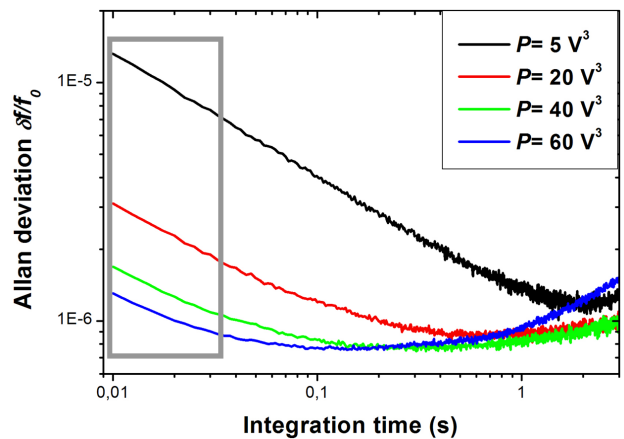
Figure 6. Allan deviation \delta f/f_0 of a crossbeam measured at ambient pressure for various products P=[V_{IN\_AC} \times V_{IN\_DC} \times V_{BIAS}] \text{ [V}^3\text{]} (the output signal is proportional to P ). In the grey region, the higher is P , the better is the resonator frequency noise as expected from [7].
