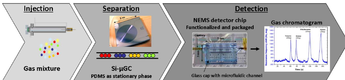
Figure 1. Schematic representation of a multi-gas analyzer associating a silicon \mu\text{GC} and NEMS detectors
