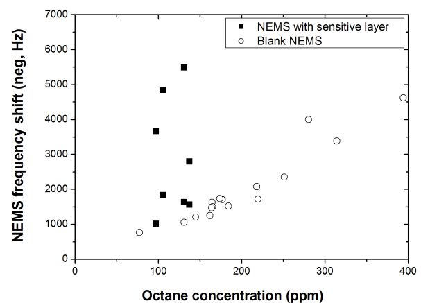
Figure 9. Example of response curves for octane: the frequency shift is plotted as a function of the concentration for several NEMS with different coating layers.
