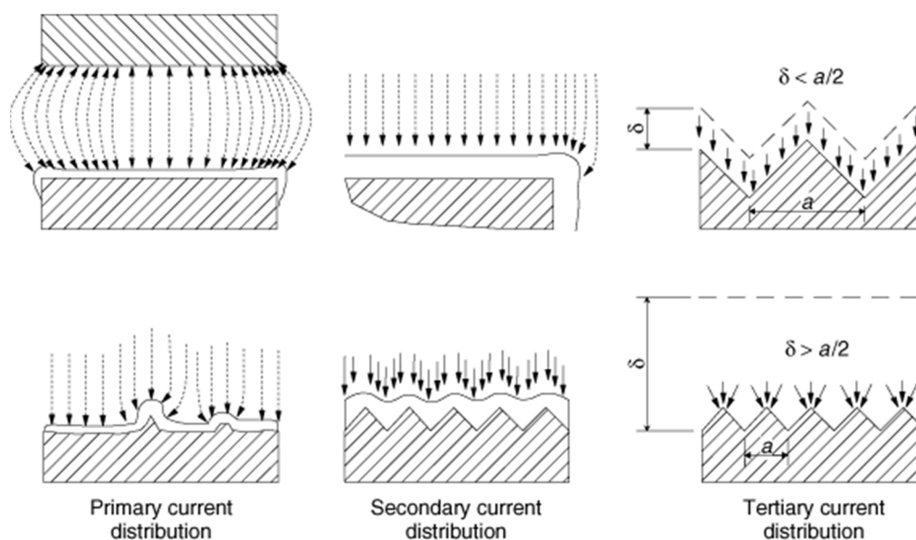
Figure 3. The effect of different current distributions (primary, secondary, and tertiary) on the electrodeposit thickness over the electrode surface. Reproduced with permission [16]. Copyright 2007, Wiley.
