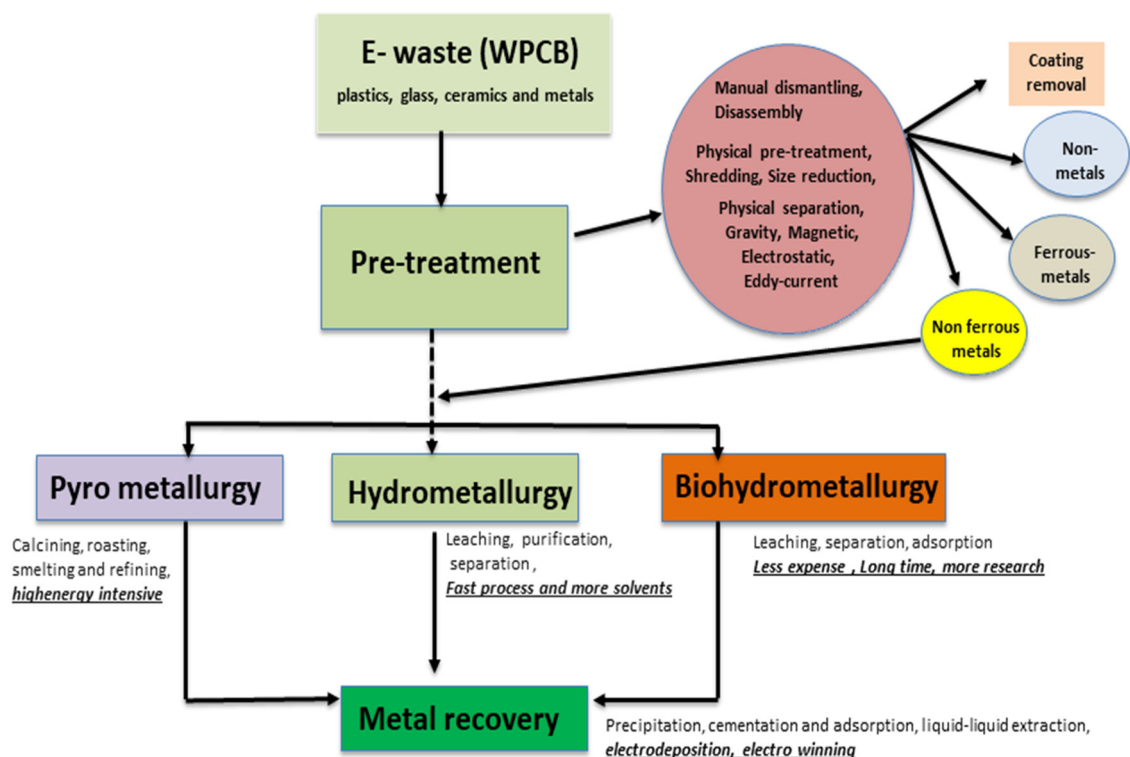
Figure 1. Scheme of metal recovery from e-waste (printed circuit boards) [9].
