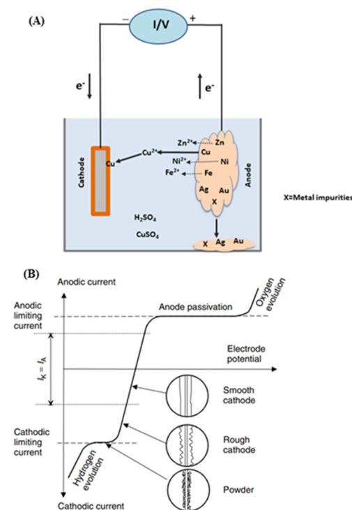
Figure 8. Schematic description of electrorefining process (A) and current density–cell voltage dependence for the electrorefining of copper (B). Reproduced with permission [16]. Copyright 2007, Wiley.
