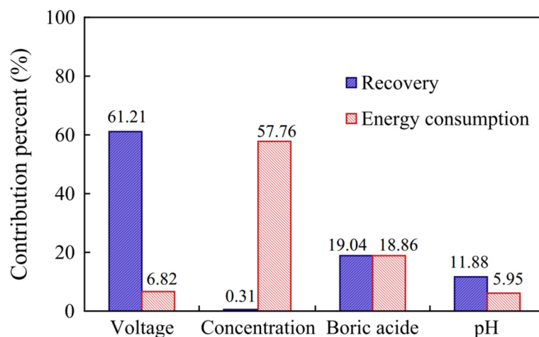
Figure 5. The contribution percent of the parameters (voltage, concentration, boric acid, and pH) of electrodeposition on Ni recovery and energy consumption. Reproduced with permission [68]. Copyright 2014, Elsevier.
