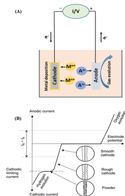
Figure 7. Schematic description of electrowinning process (A) and current density–cell voltage dependence for the electrowinning of copper (B). Reproduced with permission [16]. Copyright 2007, Wiley.
