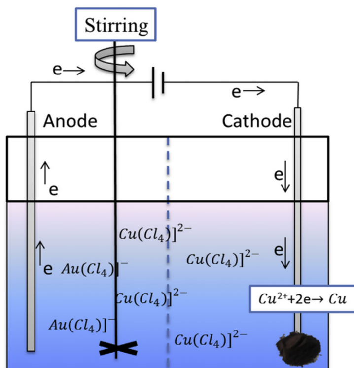
Figure 11. Schematic diagram of the electrodeposition process in HCl-NaCl-H 2 O 2 system. Reproduced with permission [81]. Copyright 2019, Elsevier.
