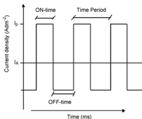
Figure 6. The typical pulse-current waveform showing T_{\text{on}} and T_{\text{off}} for one cycle. Reproduced with permission [70]. Copyright 2008, Elsevier.
