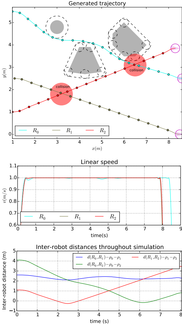
FIGURE 2. Motion planning solution without collision handling
