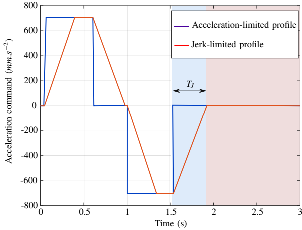
Fig. 3. Example of a jerk-limited profile. The blue zone indicate the time delay due to the shaping filter.
