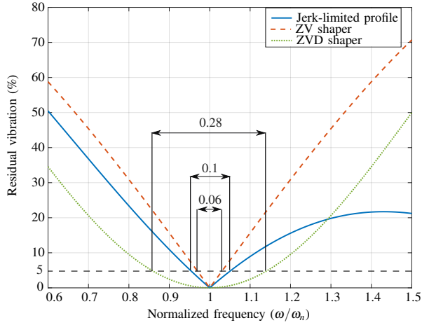
Fig. 5. Sensitivity of the residual vibration suppression action [14].
