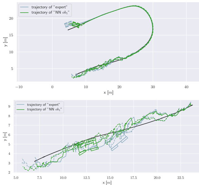
Fig. 10. The estimated paths traces by each method is set at the solid line for the rear axle, and in the dashed line the front axle. Above: the path over the full trajectory. Below: the path over the Straight segment.
