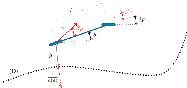
Fig. 1. The mobile robot studied.
