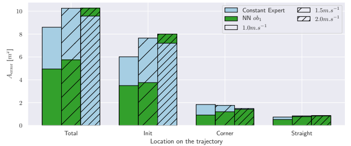
Fig. 9. The A_{\text{error}} of the tested method and the expert constant gain . The hash density show the changes in the speed.
