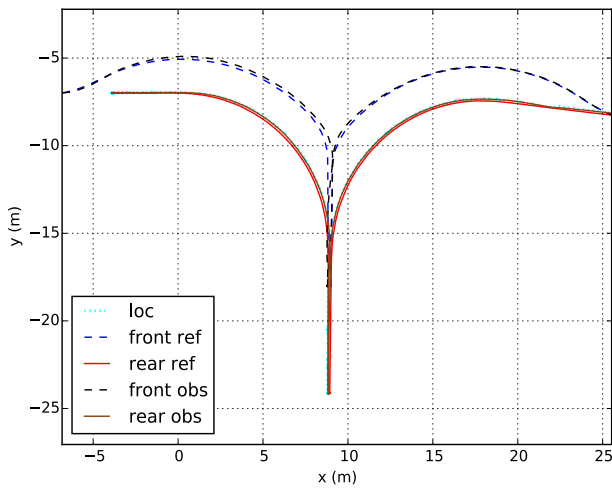
Fig. 12. Zoom on parking and departure maneuvers. (For interpretation of the references to color in this figure legend, the reader is referred to the web version of this article.)
