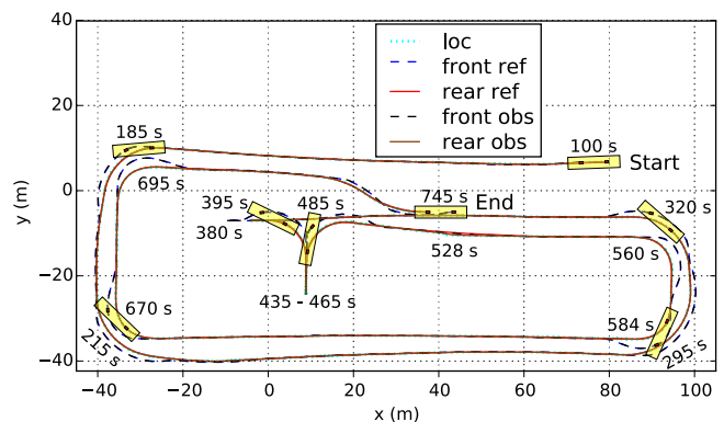
Fig. 11. Path tracking in the bus depot.
