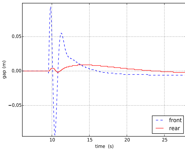
Fig. 9. Respect of lateral limits.
