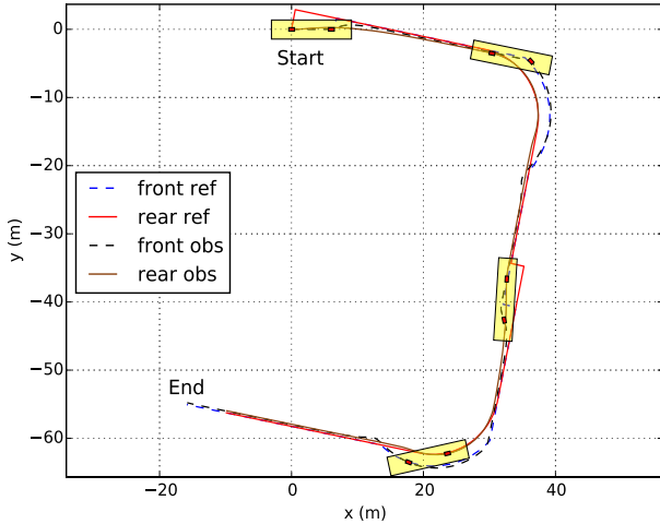
Fig. 4. U trajectory without sliding compensation.
