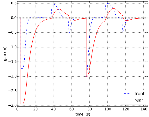
Fig. 7. Tracking error with sliding compensation.
