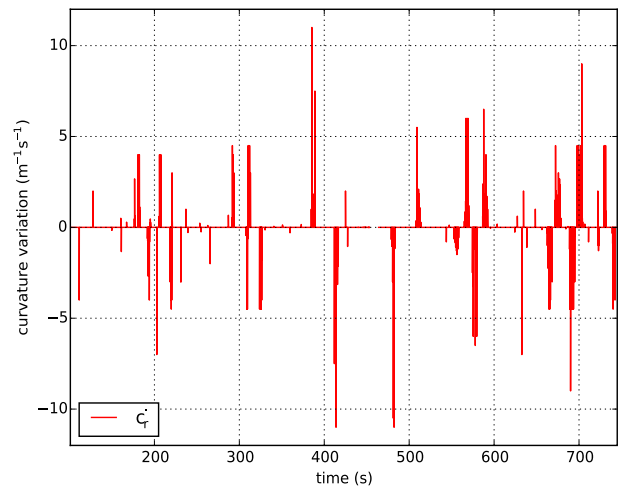
Fig. 15. Rear curvature variation.
