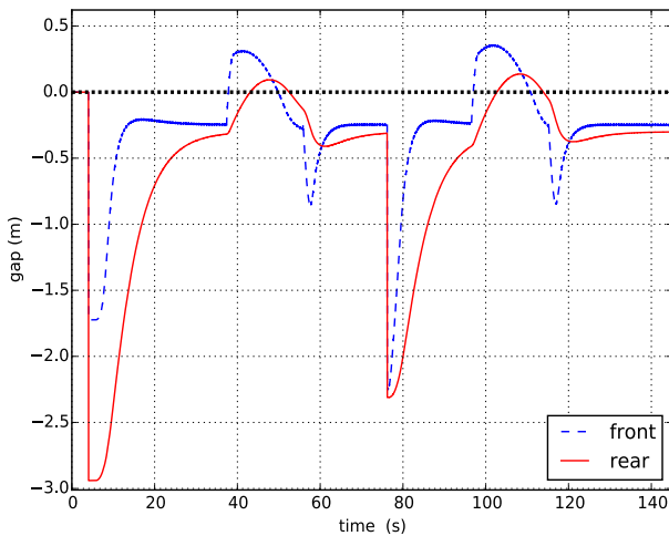
Fig. 5. Tracking error without sliding compensation.
