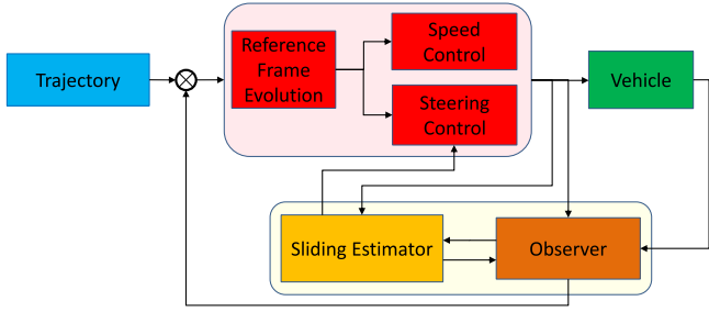
Fig. 2. Control block diagram.
