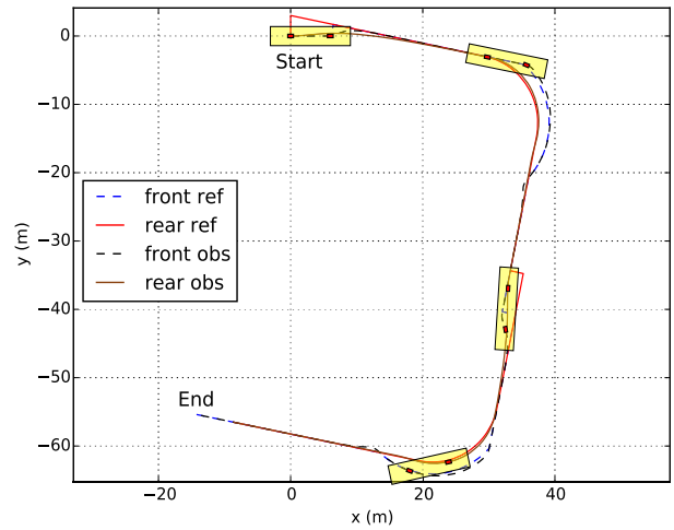
Fig. 6. U trajectory with sliding compensation.
