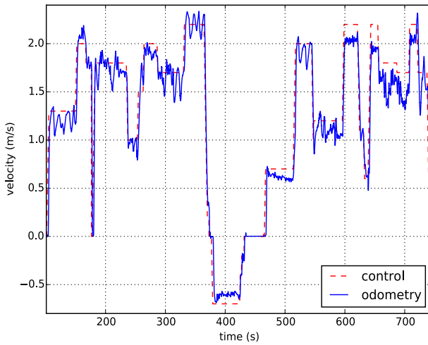
Fig. 16. Front longitudinal velocity.
