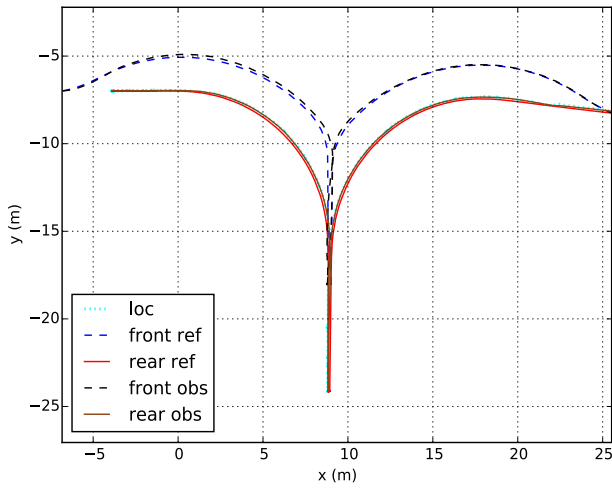
Fig. 12. Zoom on parking and departure maneuvers. (For interpretation of the references to color in this figure legend, the reader is referred to the web version of this article.)
