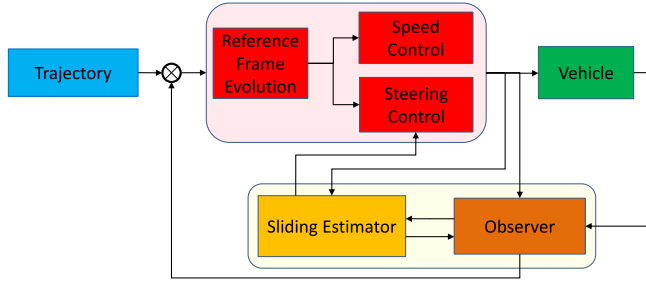
Fig. 2. Control block diagram.
