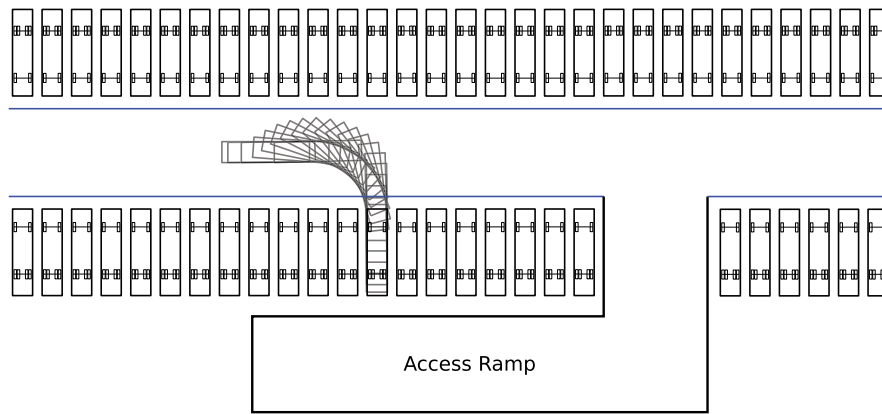
Fig. 1. Bus center configuration.
