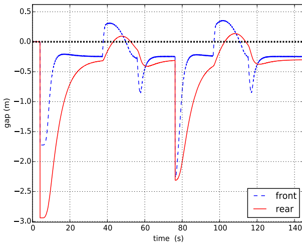
Fig. 5. Tracking error without sliding compensation.
