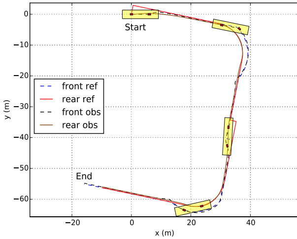
Fig. 4. U trajectory without sliding compensation.
