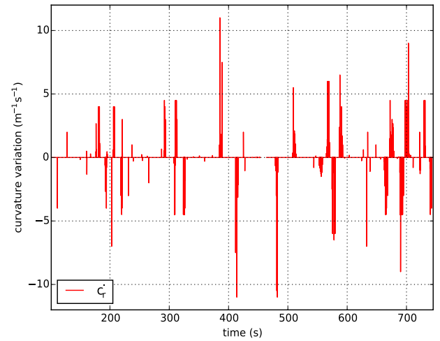
Fig. 15. Rear curvature variation.
