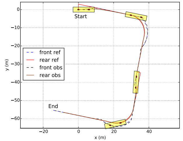
Fig. 6. U trajectory with sliding compensation.
