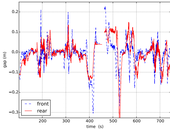
Fig. 14. Front and rear tracking errors.
