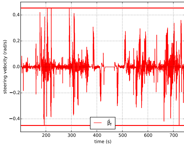
Fig. 17. Front control steering velocity.
