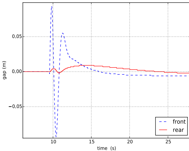
Fig. 9. Respect of lateral limits.
