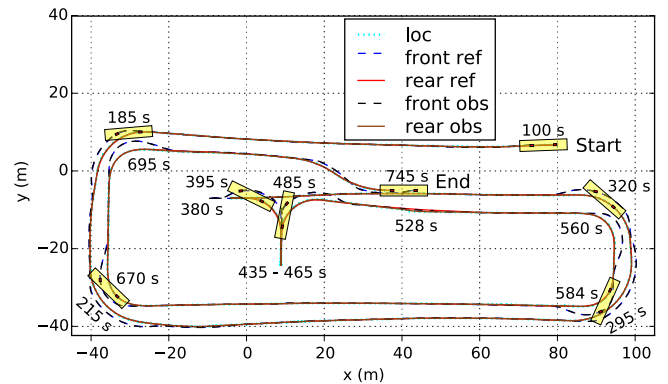
Fig. 11. Path tracking in the bus depot.
