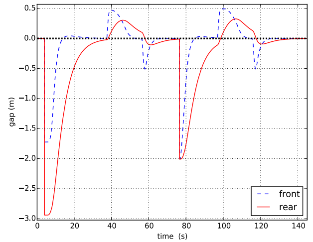
Fig. 7. Tracking error with sliding compensation.
