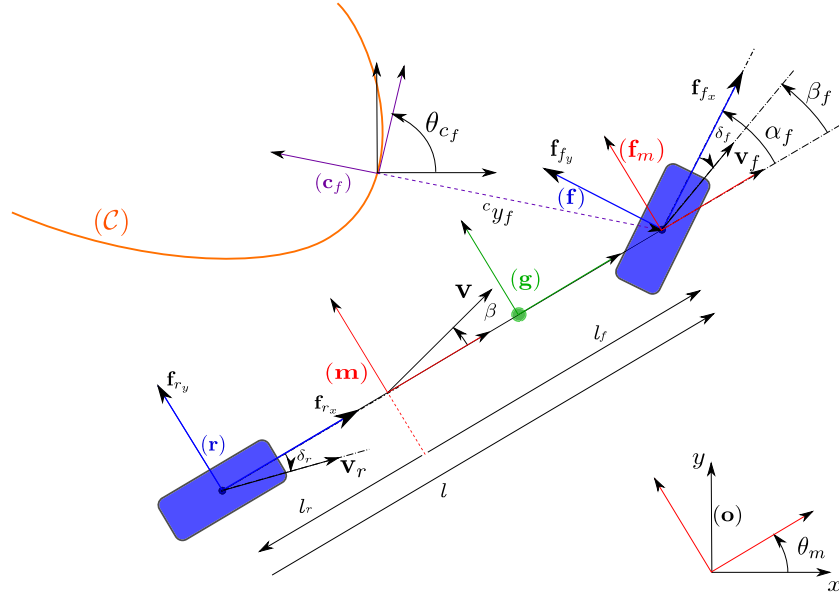
Fig. 3. Planar horizontal model.
