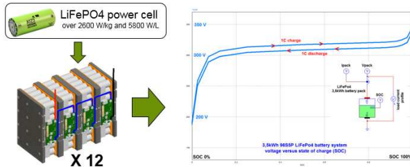
Fig. 7: Battery pack design
